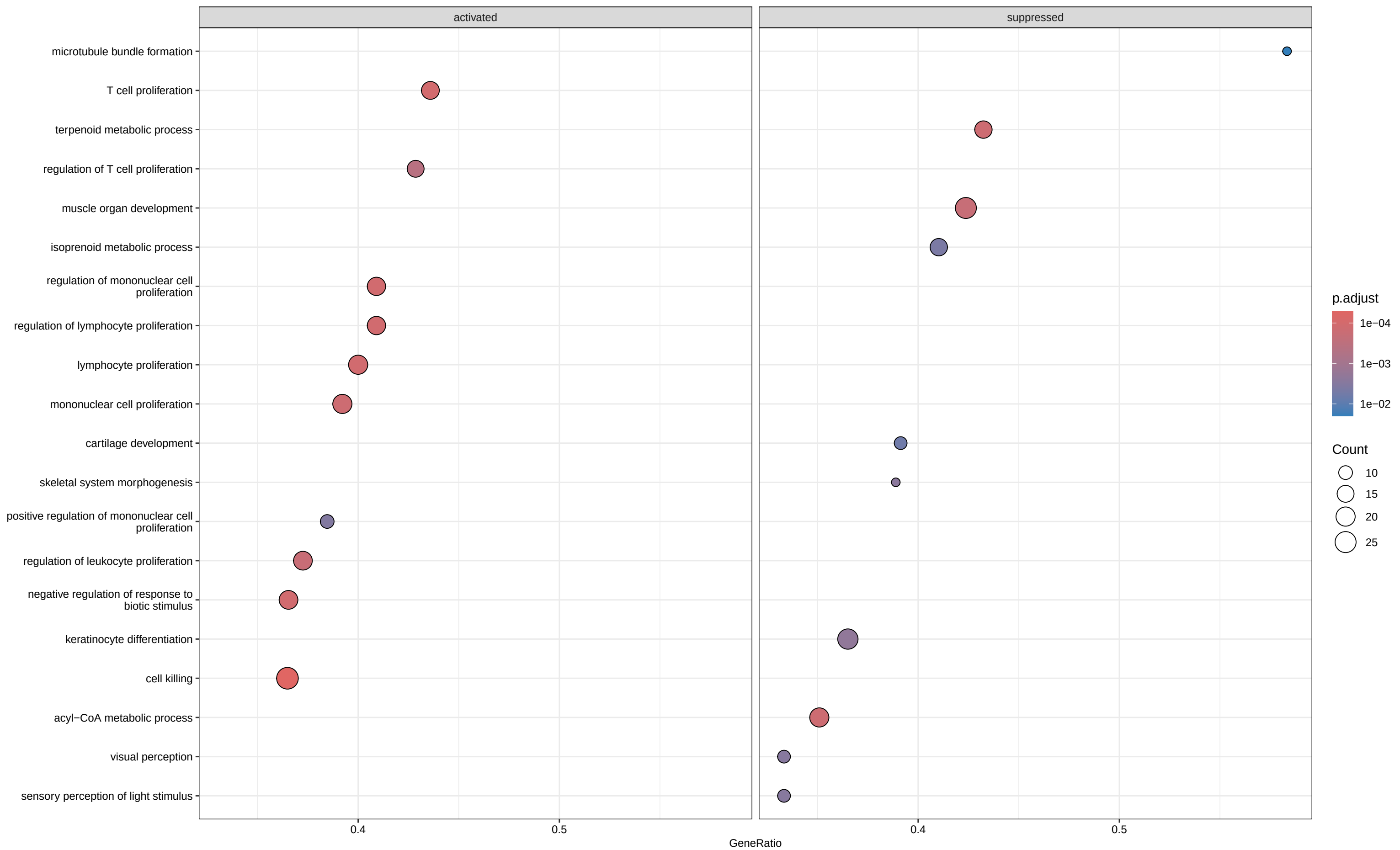
LC vs Healthy: GSEA GO BP top pathways
