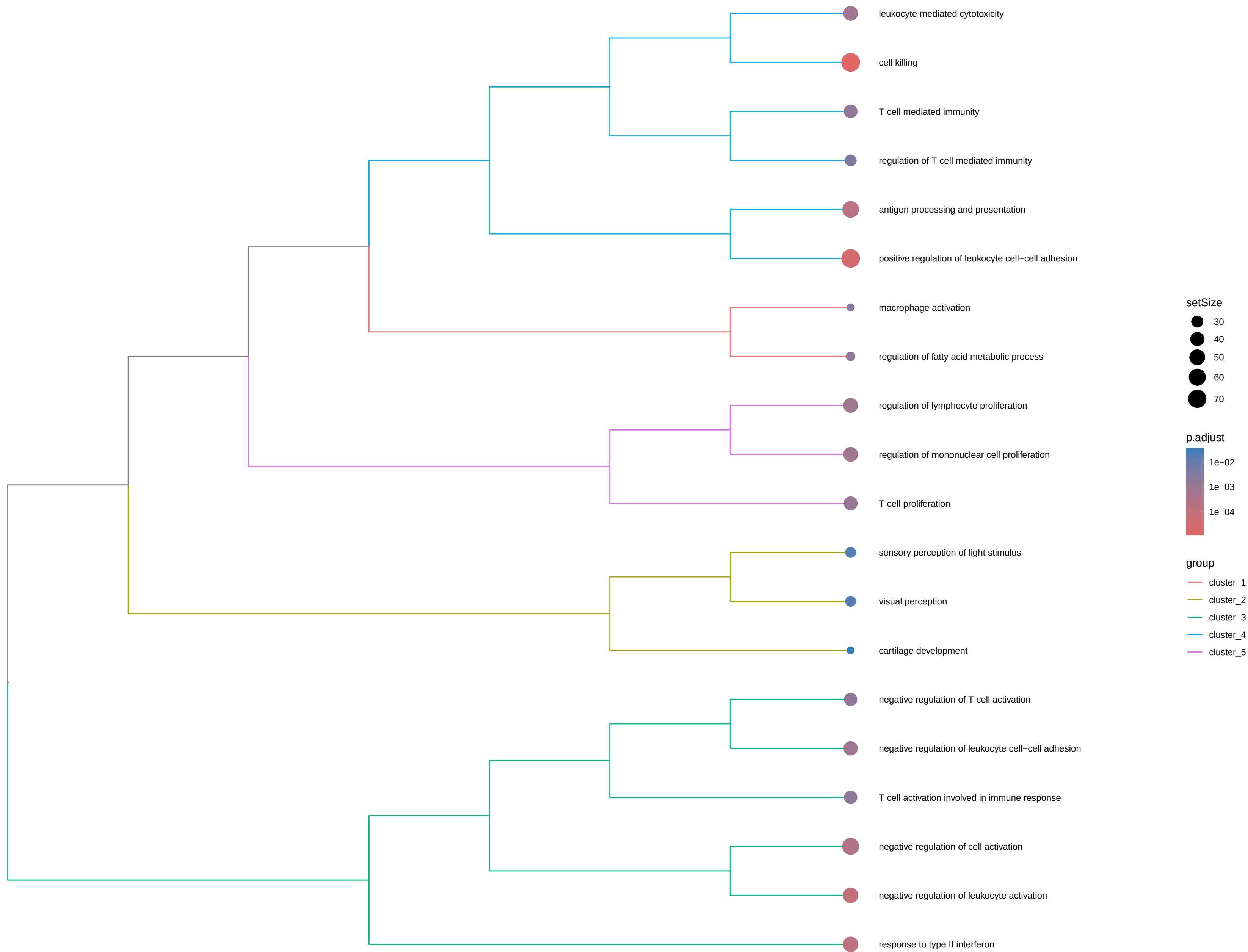
FC vs Healthy: GSEA GO BP tree plot
