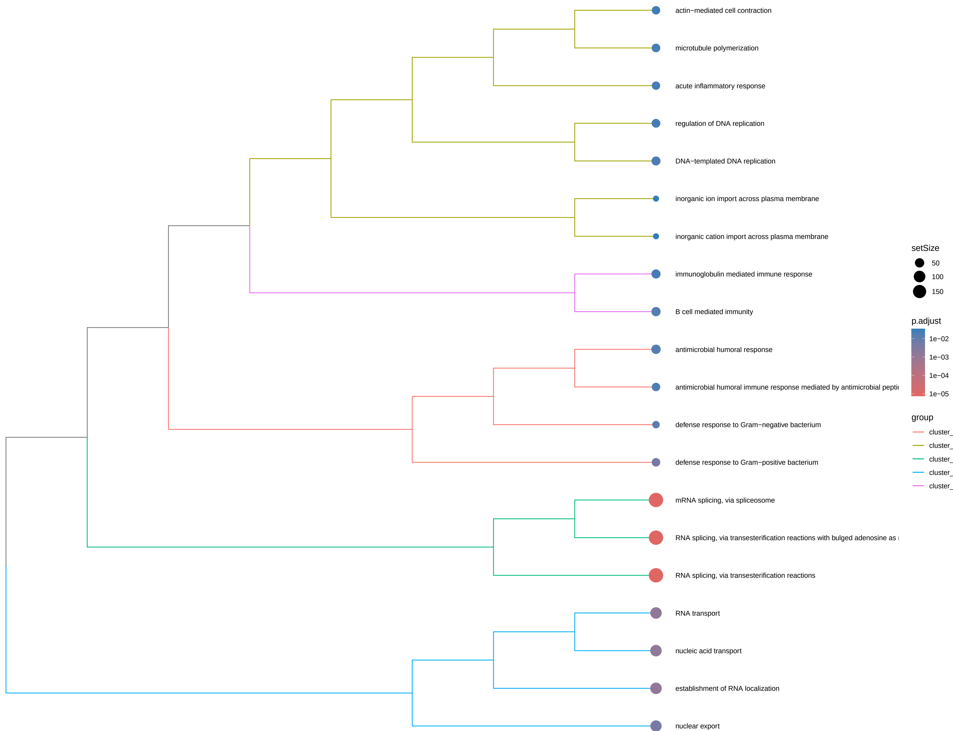
LC vs FC: GSEA GO BP tree plot
