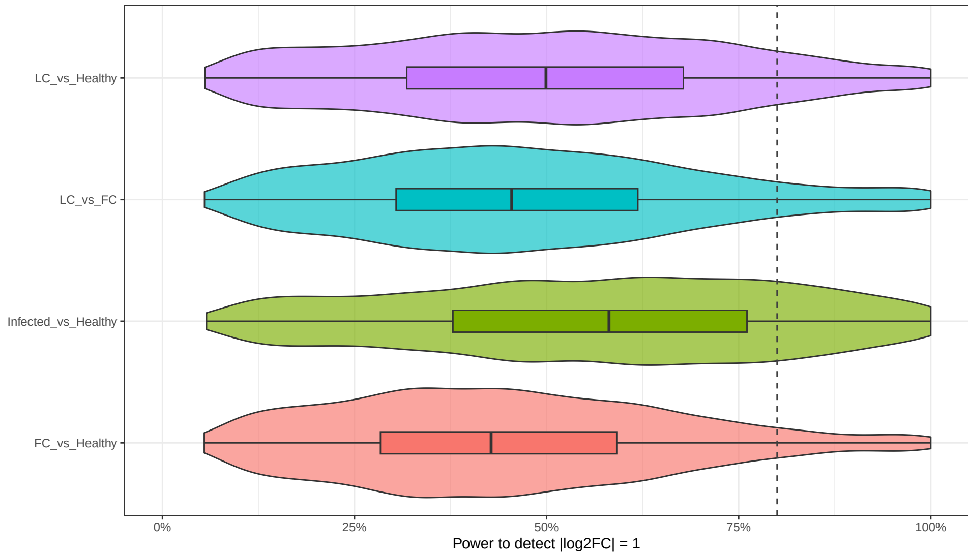
Power for the target effect size by comparison
