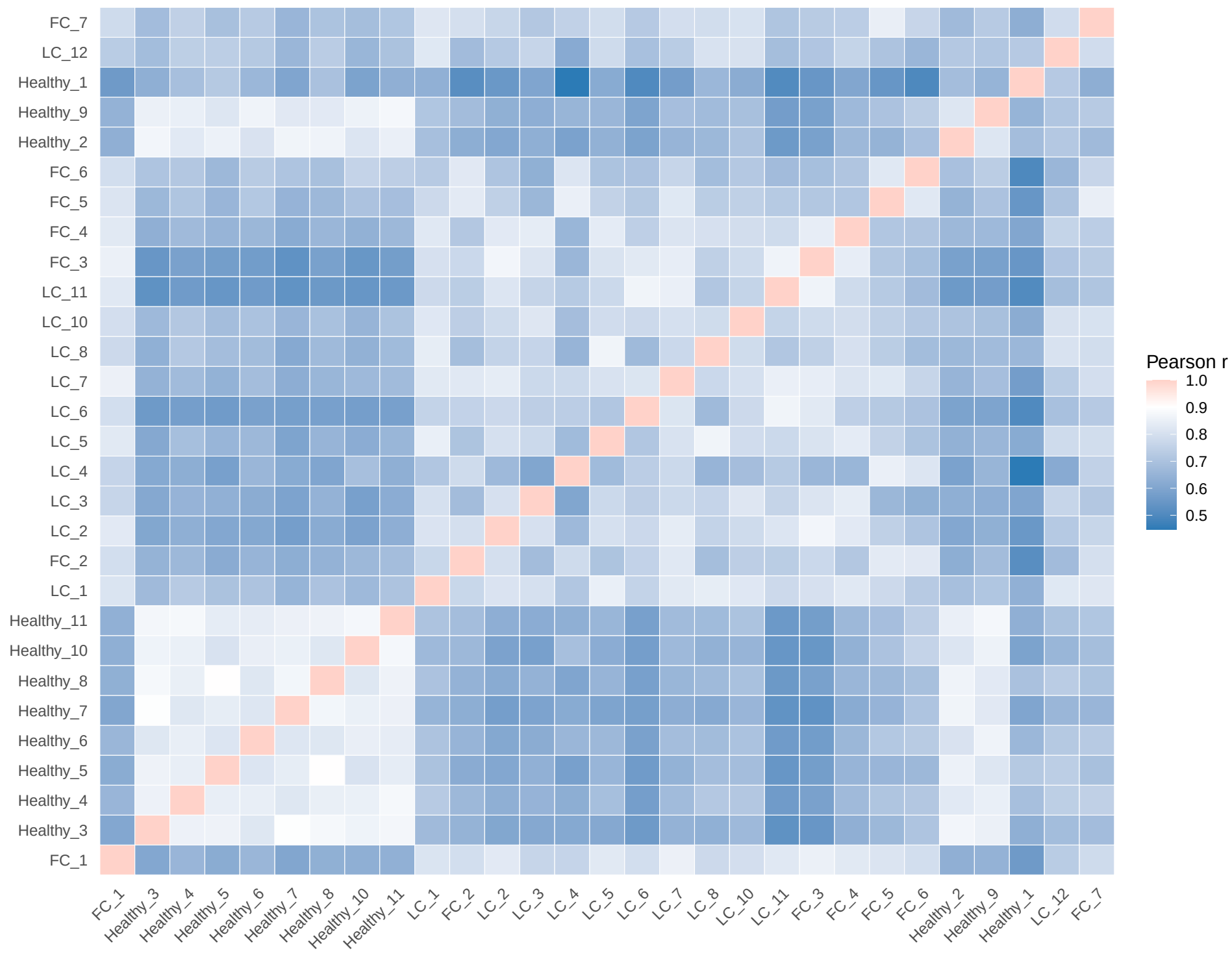
MSstats protein-level correlation between samples
