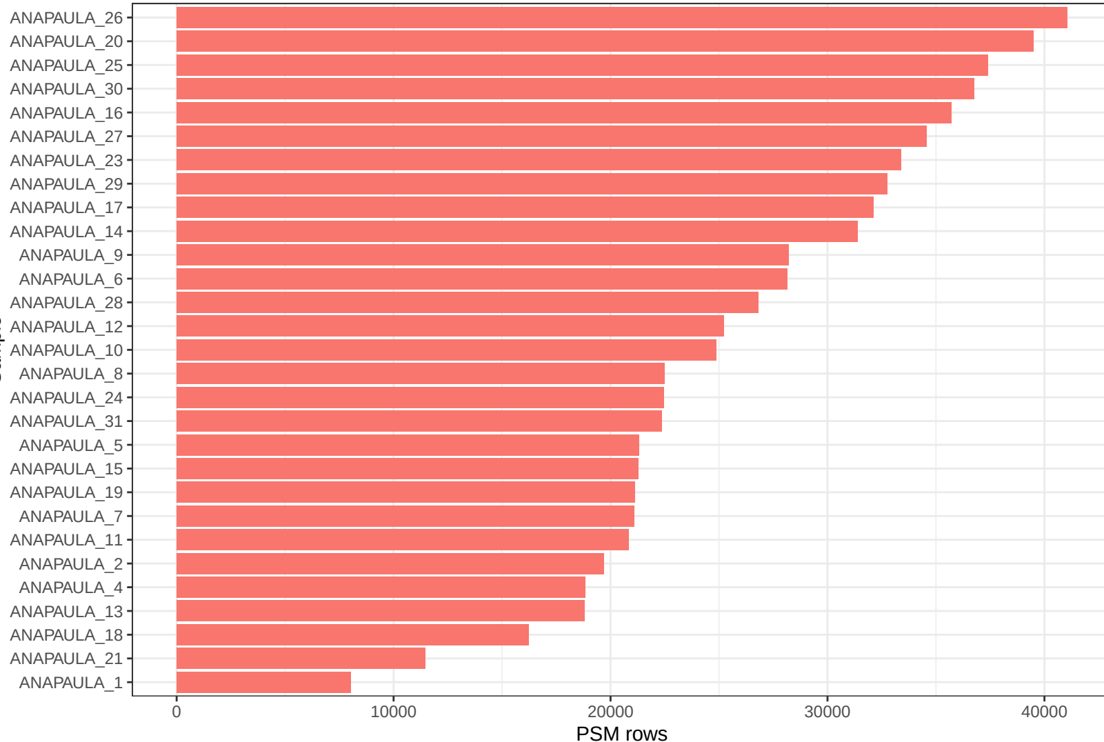
Raw PSM intensity status per sample
