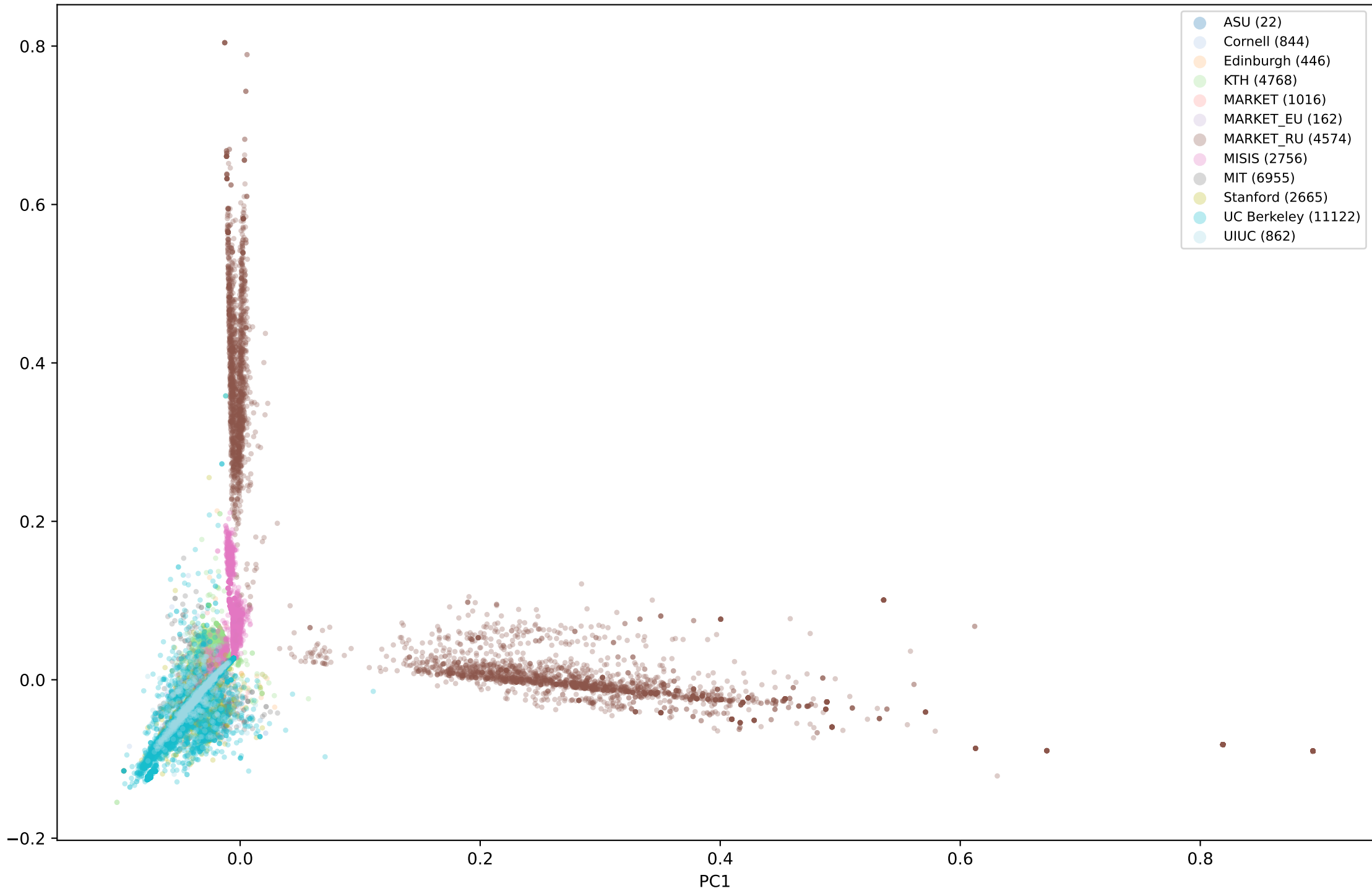
ADS Latent Space: PCA by Institution
