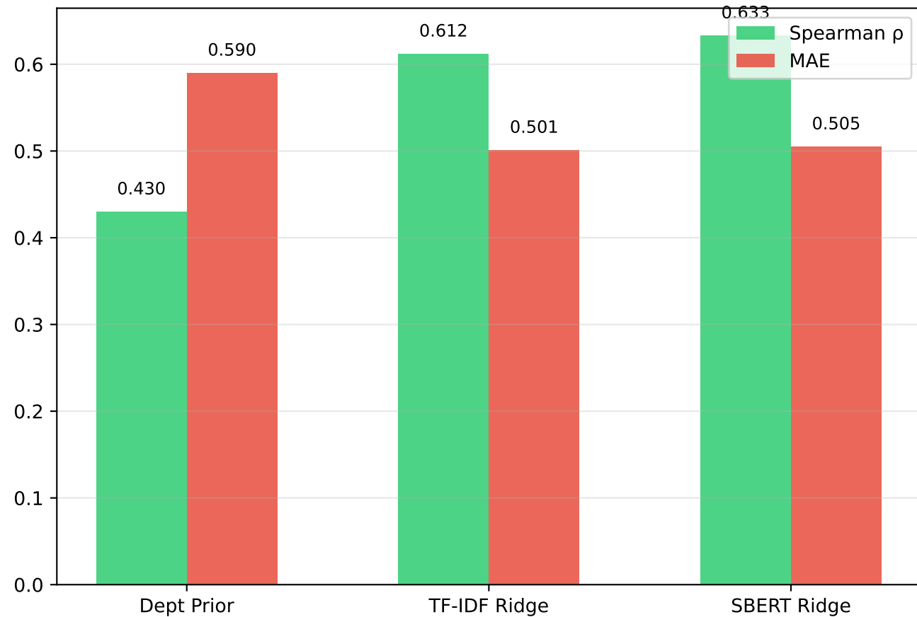
Task 1: Richness Prediction
