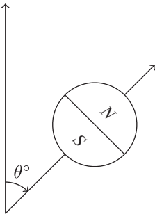
Figure 1.6 Electron with spin N in the \theta^\circ direction.
