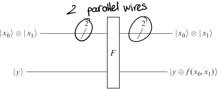
Figure 9.1 The oracle for f .
