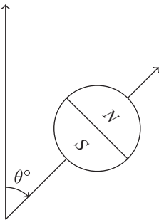
Figure 1.6 Electron with spin N in the \theta^\circ direction.
