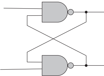
Figure 6.11 A flip-flop using two NAND gates.
