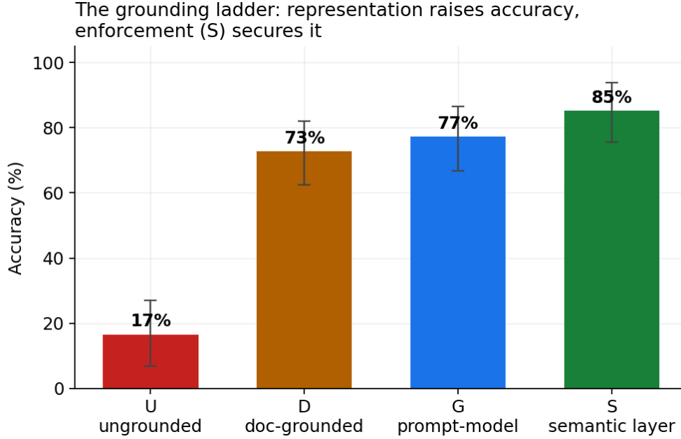
Figure 1: The grounding ladder. Accuracy pooled across the five complete-coverage models and two datasets, with 95% cluster-bootstrap confidence intervals (partial single-run tiers excluded). Representation (U→G) delivers the bulk of the gain; enforcement (G→S) secures it.
