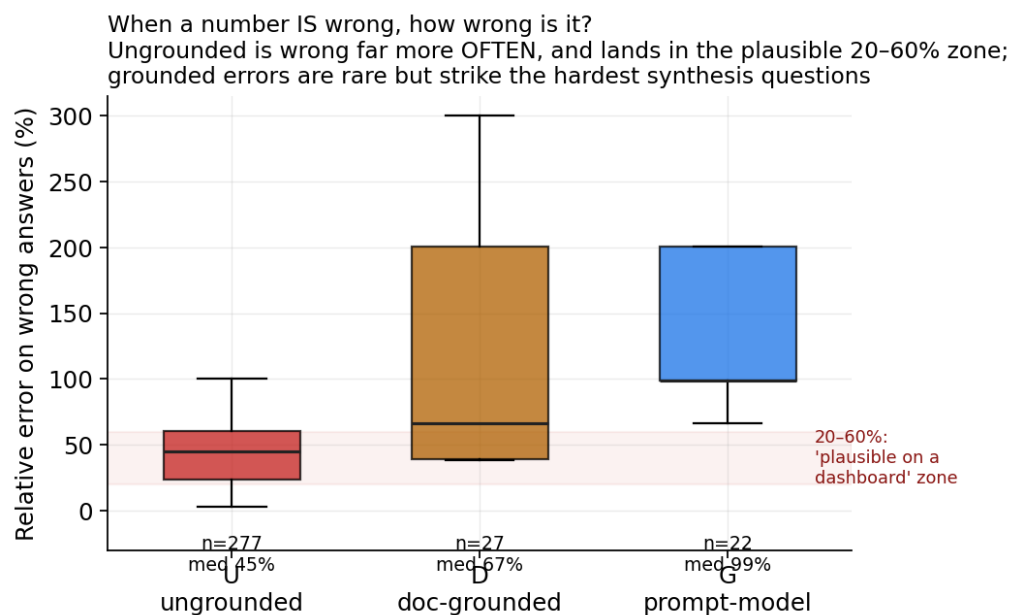
Figure 7: Relative error on wrong numeric answers, by condition, over the 5 complete-coverage models (n per box annotated; 326 wrong-with-error across conditions — a full-CSV recount including the two partial tiers gives 338 for U, same story). The ungrounded condition is wrong far more often and its errors cluster in the 20–60% “plausible on a dashboard” zone — off enough to mislead, close enough to escape notice. The grounded conditions are wrong rarely, but when they are it is on the hardest synthesis questions, where the few errors are large. Being wrong less often and being wrong by a plausible-looking margin are different risks; ungrounded analytics carries both.
