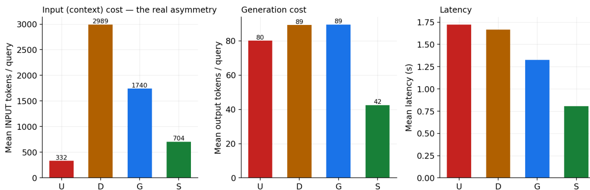
Figure 9: Cost by condition (Gemini arm). The asymmetry is input-side : D resends a ~2989-token knowledge base on every call and G a ~1740-token model, while S sends a compact ~704-token field catalog; S also emits the fewest output tokens and has the lowest latency.
