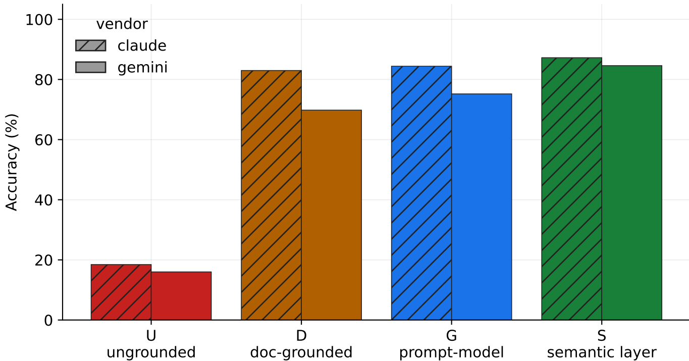
The ladder holds across vendors (solid = Gemini, hatched = Claude)
