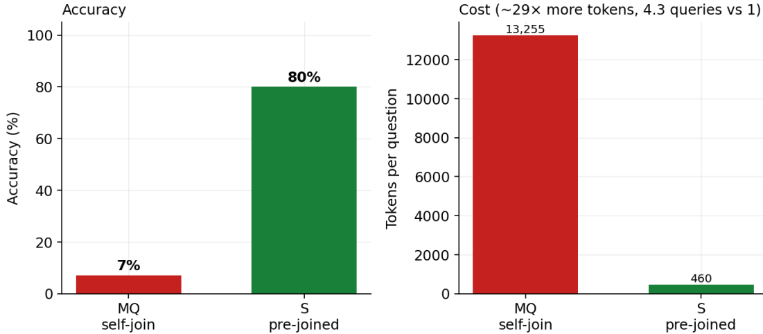
Figure 5: Model-orchestrated multi-query self-join (MQ) vs. the pre-joined semantic layer (S): accuracy, and cost per question.
