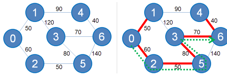
Figure 4.13: Minimax (UVa 10048 [44])
