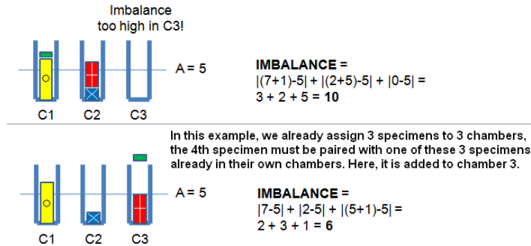
Figure 3.8: UVa 00410 - Observations
