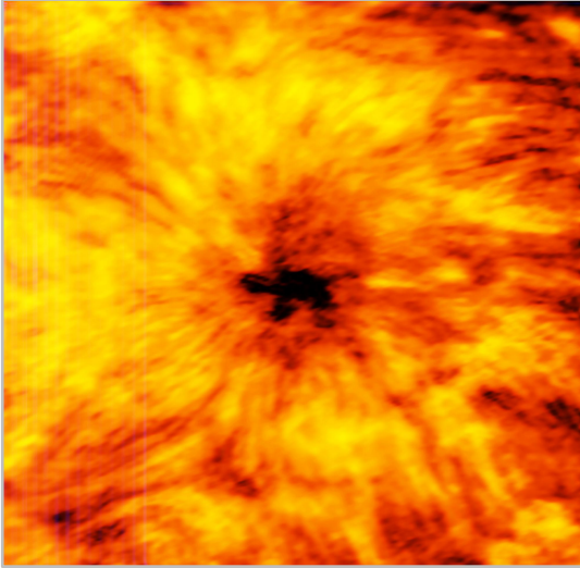
Sunspot at 1.25 mm
