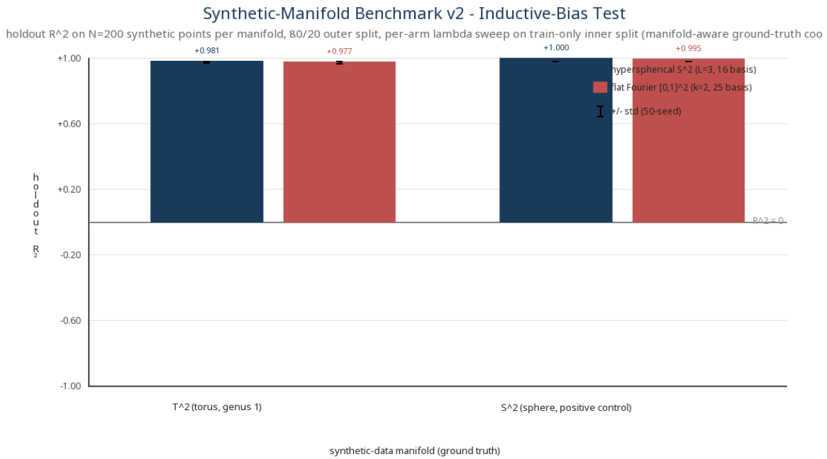
Figure C.2. Synthetic-manifold benchmark v2 — 50-seed holdout R^2 on N=200 synthetic points per manifold, manifold-aware ground-truth coordinates, per-arm \lambda sweep on a train-only inner split, bars drawn from the R^2=0 baseline. Bars show mean; error bars show \pm std. The sphere wins on S^2 ( +1.0000 \pm 0.0000 vs flat's +0.9948 \pm 0.0018 , paired p < 0.0001 , sphere 50/50) as predicted. On T^2 the sphere also wins ( +0.9814 \pm 0.0110 vs flat's +0.9765 \pm 0.0085 , paired p = 0.0112 favoring sphere, sphere 37/50); the v1 prediction (flat wins on T^2 ) reverses under the clean v2 protocol.
