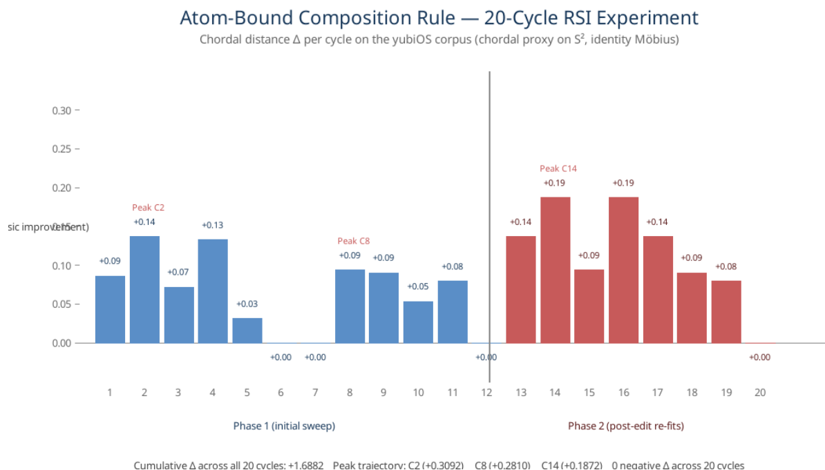
Figure 4. \mathcal{D} per cycle across the 20-cycle atom experiment. Blue: initial corpus sweep (cycles 1–12). Red: post-edit re-fits (cycles 13–20). Stars mark the three peak runs (C2, C8, C14). Cumulative \mathcal{D} across all 20 cycles: +1.6882. Zero negative \mathcal{D} across 20 cycles confirms the atom's invariant (Lemma 1).
