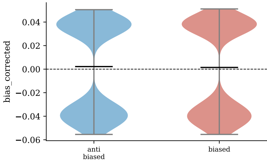
Gender_identity — bias score violin by label
