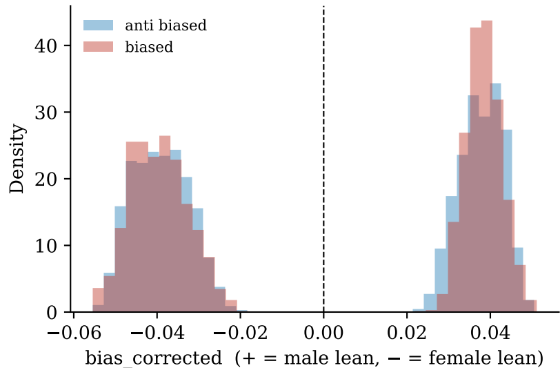
Gender_identity — bias axis projection by label
