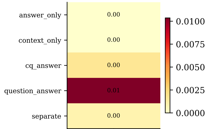
|Cohen's d| PC1
