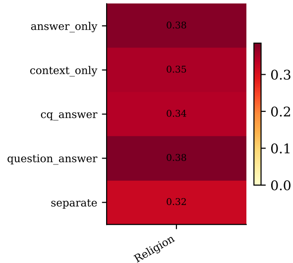
Accuracy
