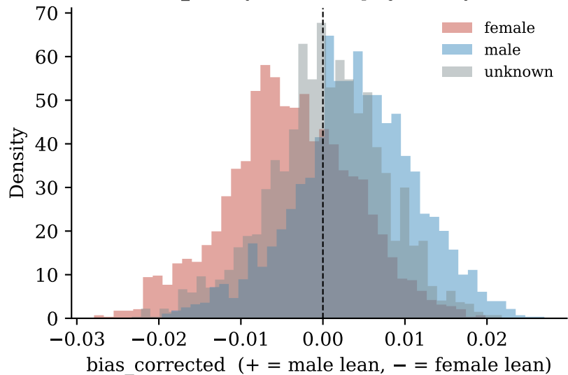
Gender_identity — bias axis projection by label
