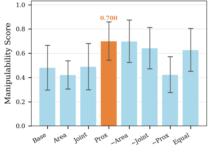
Fig. 4. Mean manipulability score ( \pm 1 std.) for each of the eight cost configurations. Configurations that include the proximity term (Prox, ~Area, ~Joint, Equal) consistently achieve higher dexterity. Best configuration highlighted in orange.
