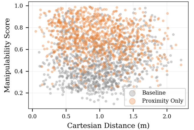
Fig. 7. Manipulability score vs. Cartesian goal distance for the baseline (grey) and proximity-only (orange) configurations. Each point represents one successful plan.
