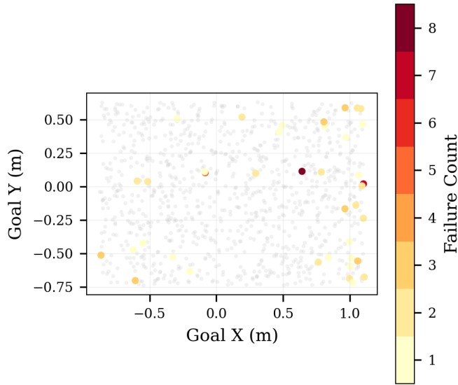
Fig. 9. Goal difficulty heatmap. Each of 1,000 goals is colored by the number of cost configurations (out of 8) that failed to find a plan.
