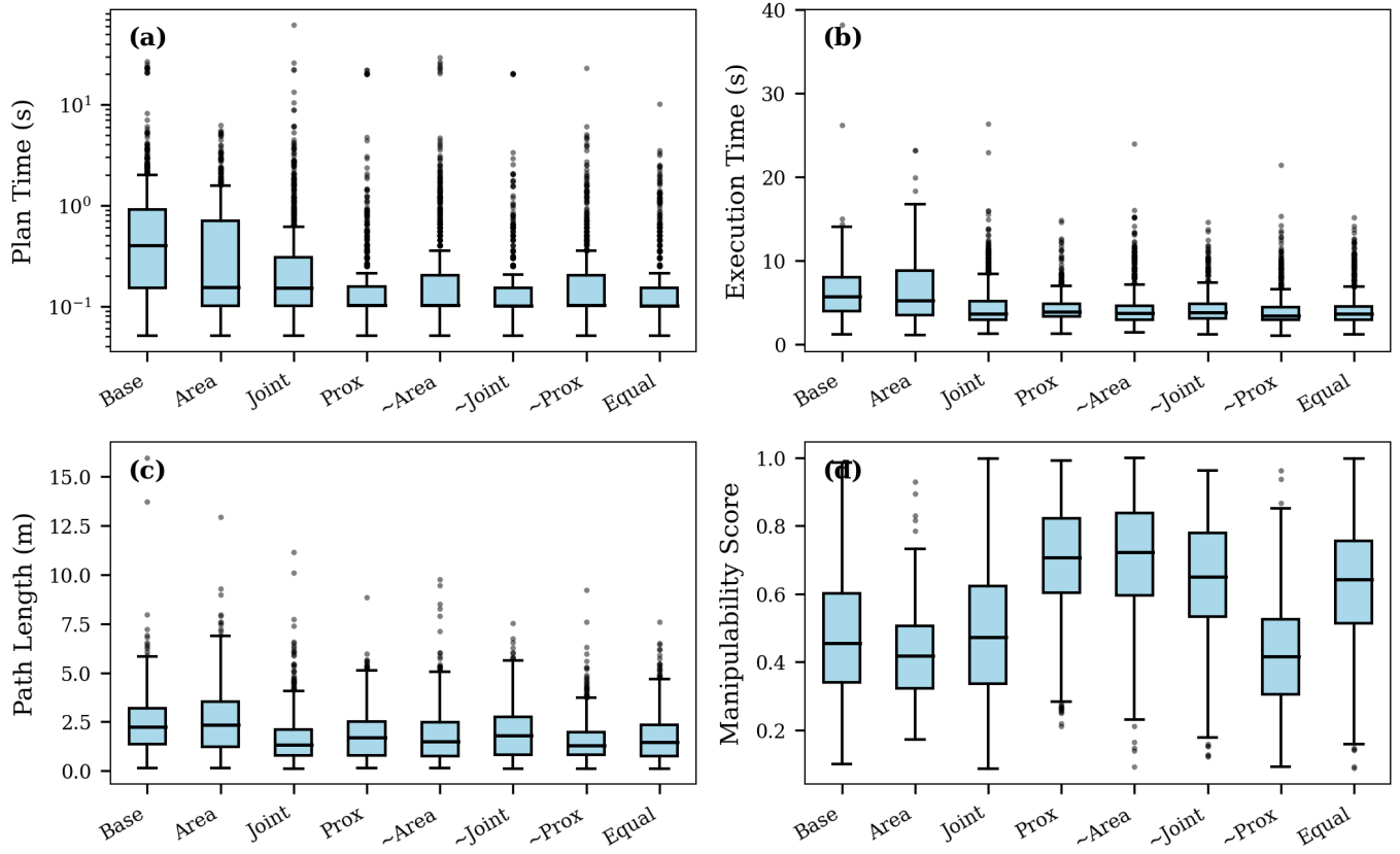
Fig. 8. Per-goal distributions across eight cost function configurations. (a) Plan time (log scale), (b) execution time, (c) path length, (d) manipulability score. All metrics computed over successful plans only.
