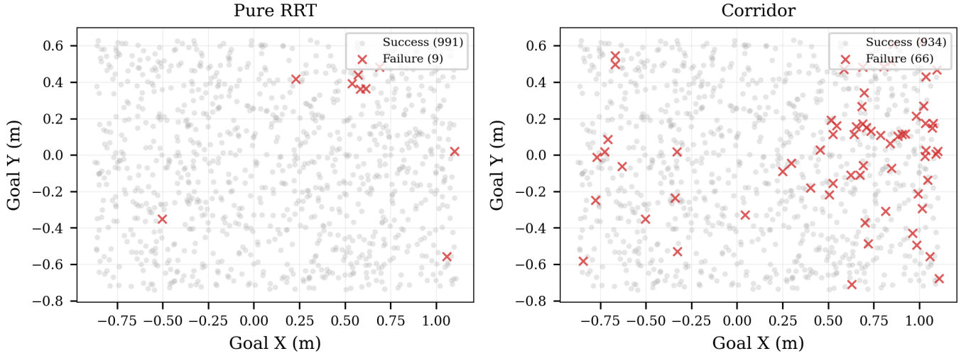
Fig. 6. Spatial distribution of planning failures. Left: unconstrained RRT (9 failures). Right: corridor-constrained planning (66 failures), with failures concentrated at the workspace boundary.
