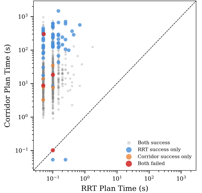
Fig. 5. Per-goal plan time comparison. Each point represents one of 1,000 goals. Points above the diagonal indicate corridor planning was slower.
