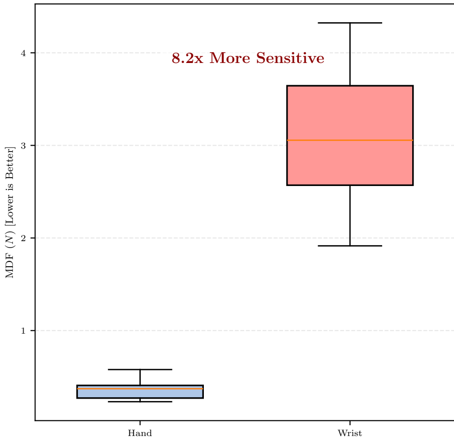
Fig. 1: Minimum Detectable Force (Sensitivity)
