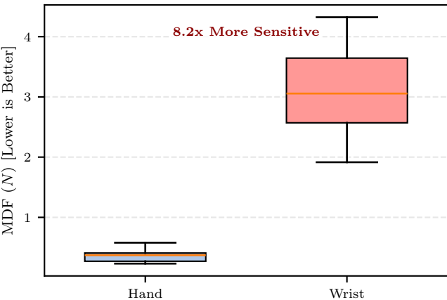
Fig. 1: Minimum Detectable Force (Sensitivity)
