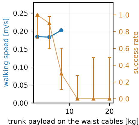
(b) trunk payload, n = 10
