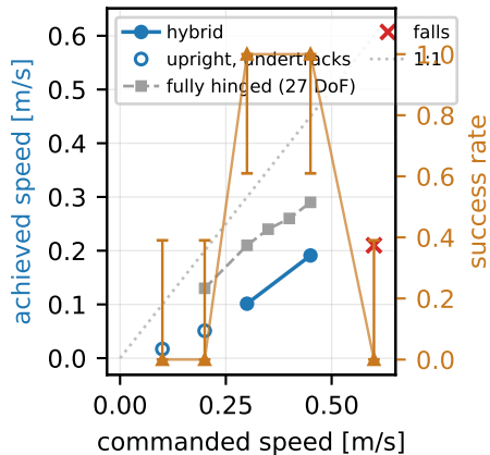
(a) speed envelope, n = 6
