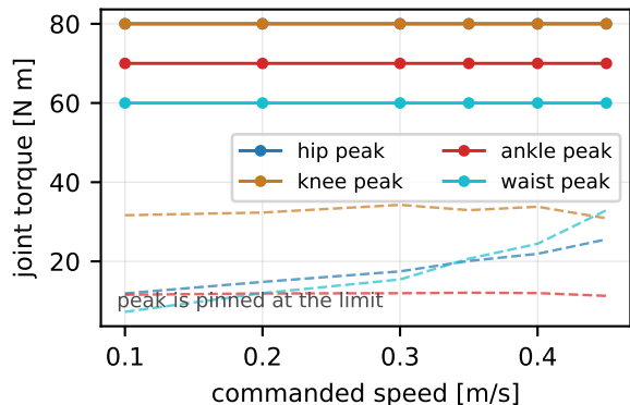
peak (solid) and RMS (dashed) joint torque
