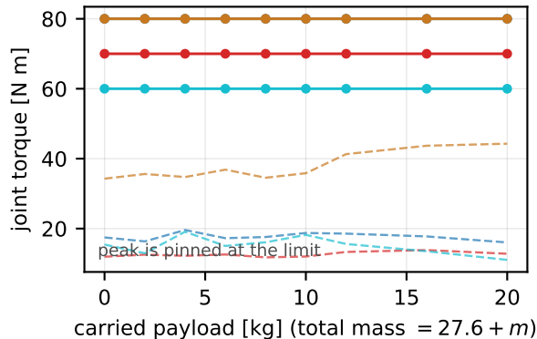
peak (solid) and RMS (dashed) joint torque
