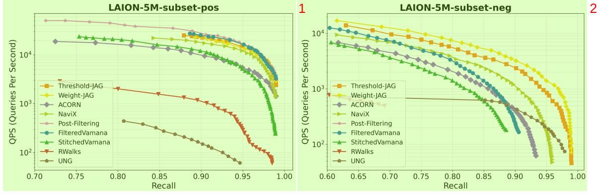
Figure 6. QPS vs. recall plots for subset filters with positive and negative correlations on the LAION-5M dataset. 3
