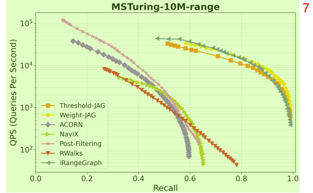
Figure 1. QPS vs. recall plot for range filters on the MSTuring-10M dataset. Please refer to Section 4 for experimental details.
