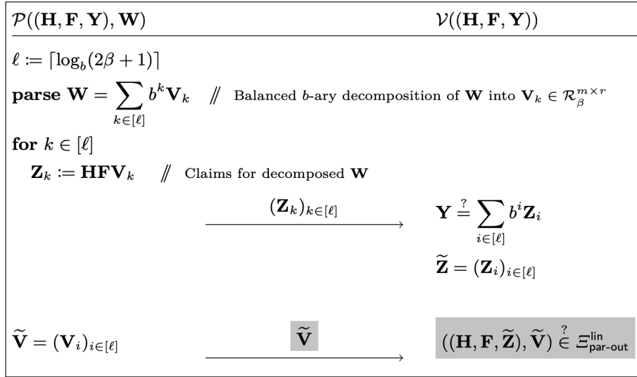
Fig. 3. Protocol \Pi^{b\text{-decomp}} , a reduction of \Xi_{\text{par-in}}^{\text{lin}} to \Xi_{\text{par-out}}^{\text{lin}} with par-in, par-out specified in Lemma 4. As a proof (but not reduction ) of knowledge, \Pi^{b\text{-decomp}} sends the marked parts.
