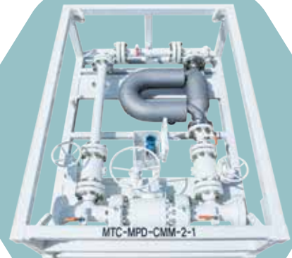
2K Coriolis-Meter-Manifold
