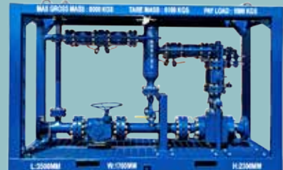
Sample-Catcher-Manifold
