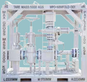
NSD Manifold
