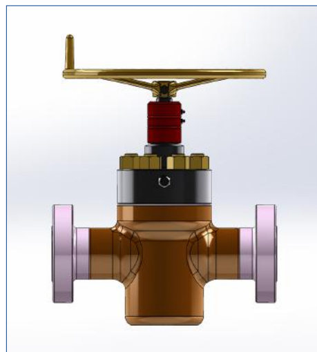
One Piece Seat and Gate with Wedge Guide Design
