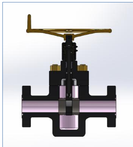
Model 500 Gate Valve
