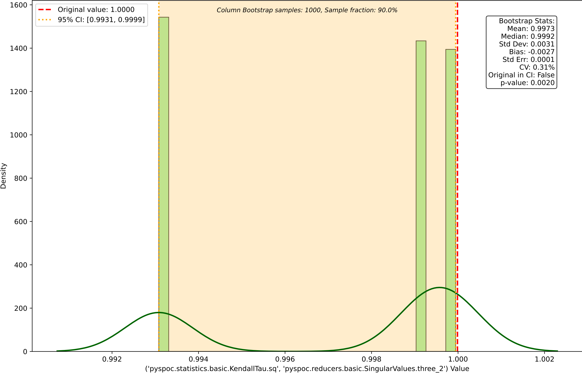
Column Bootstrap Distribution for ('pyspoc.statistics.basic.KendallTau.sq', 'pyspoc.reducers.basic.SingularValues.three_2')
