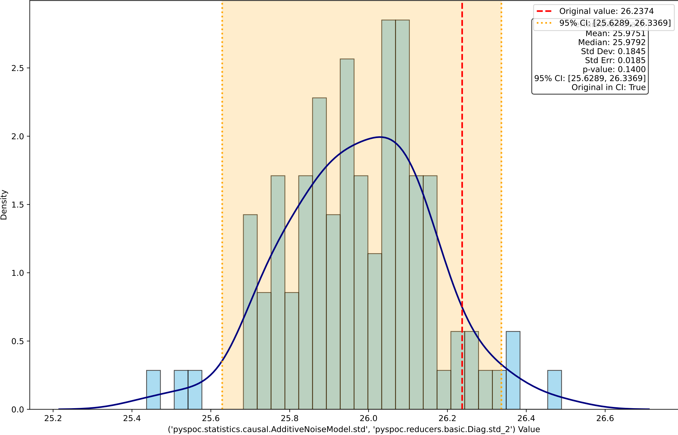
Perturbation Distribution for ('pyspoc.statistics.causal.AdditiveNoiseModel.std', 'pyspoc.reducers.basic.Diag.std_2')
