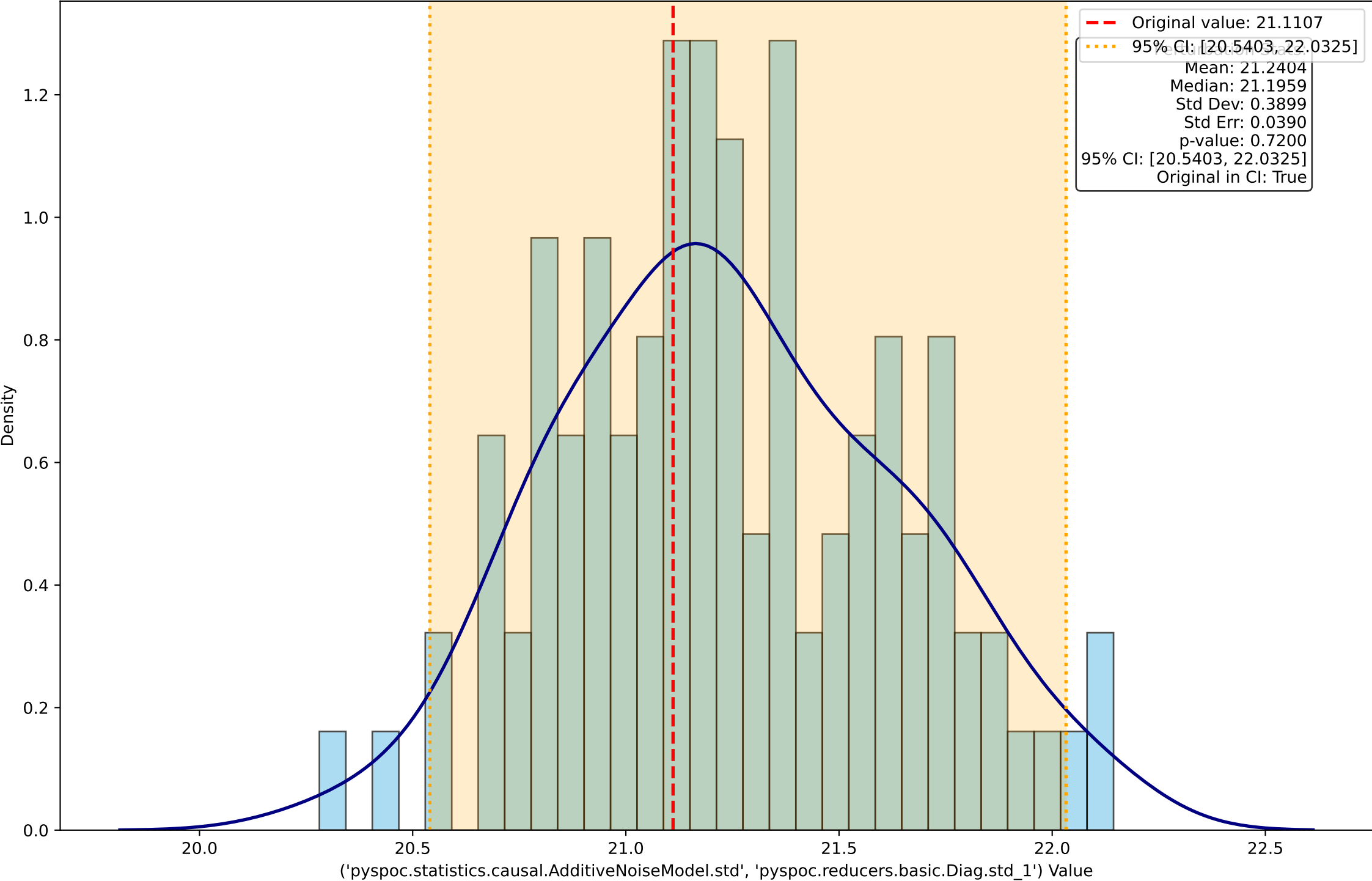
Perturbation Distribution for ('pyspoc.statistics.causal.AdditiveNoiseModel.std', 'pyspoc.reducers.basic.Diag.std_1')
