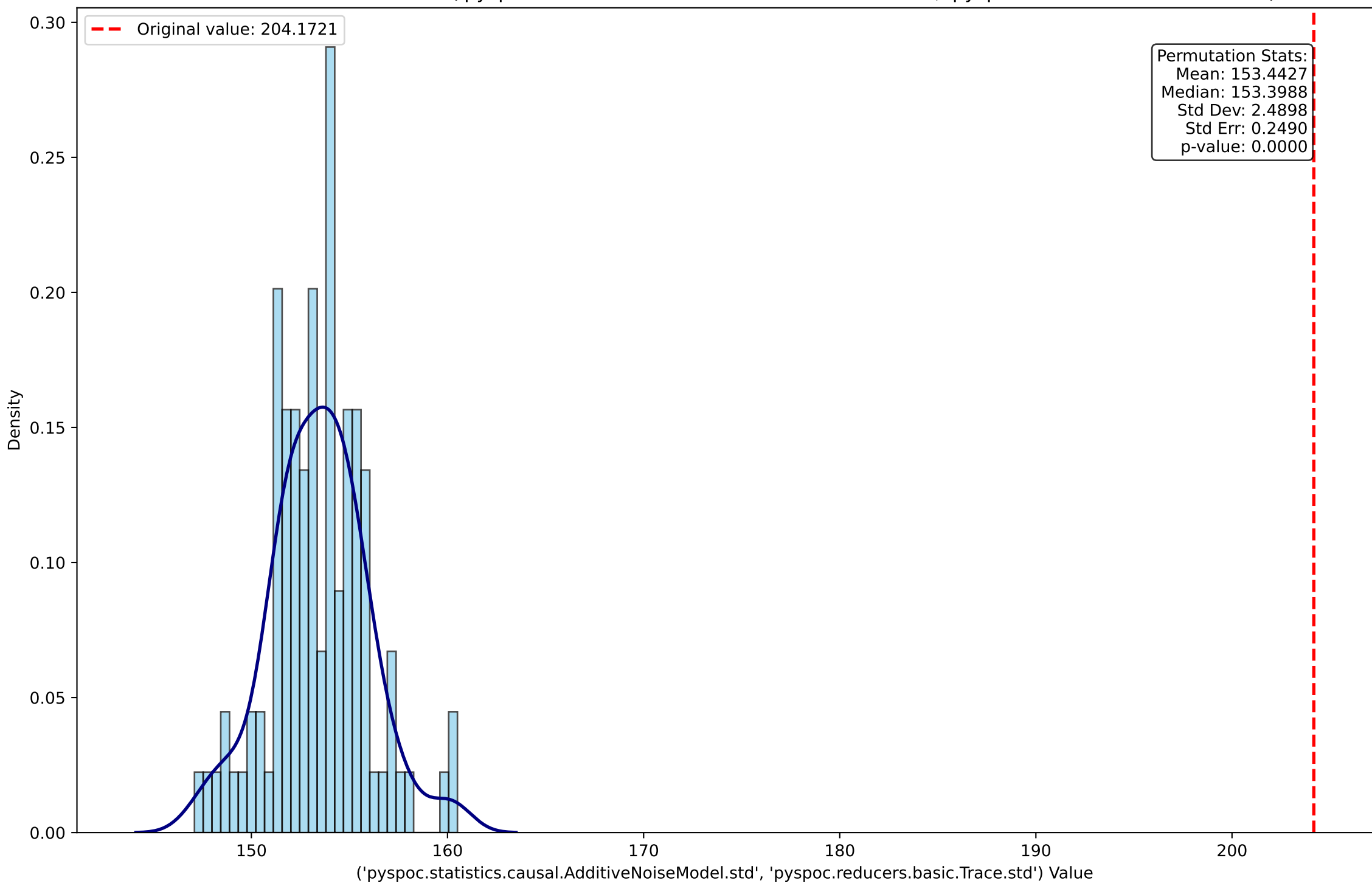
Permutation Distribution for ('pyspoc.statistics.causal.AdditiveNoiseModel.std', 'pyspoc.reducers.basic.Trace.std')
