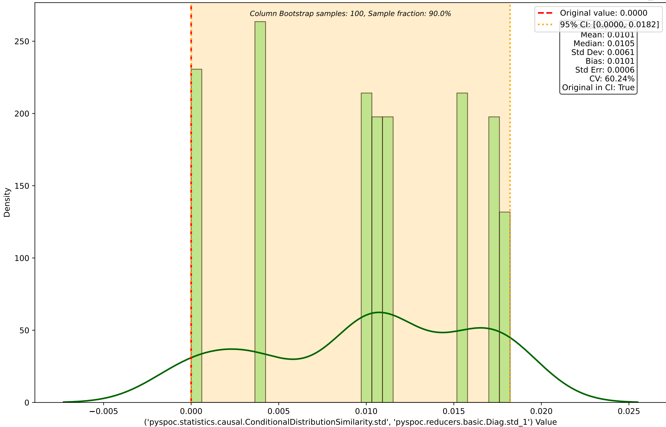
Column Bootstrap Distribution for ('pypoc.statistics.causal.ConditionalDistributionSimilarity.std', 'pypoc.reducers.basic.Diag.std_1')
