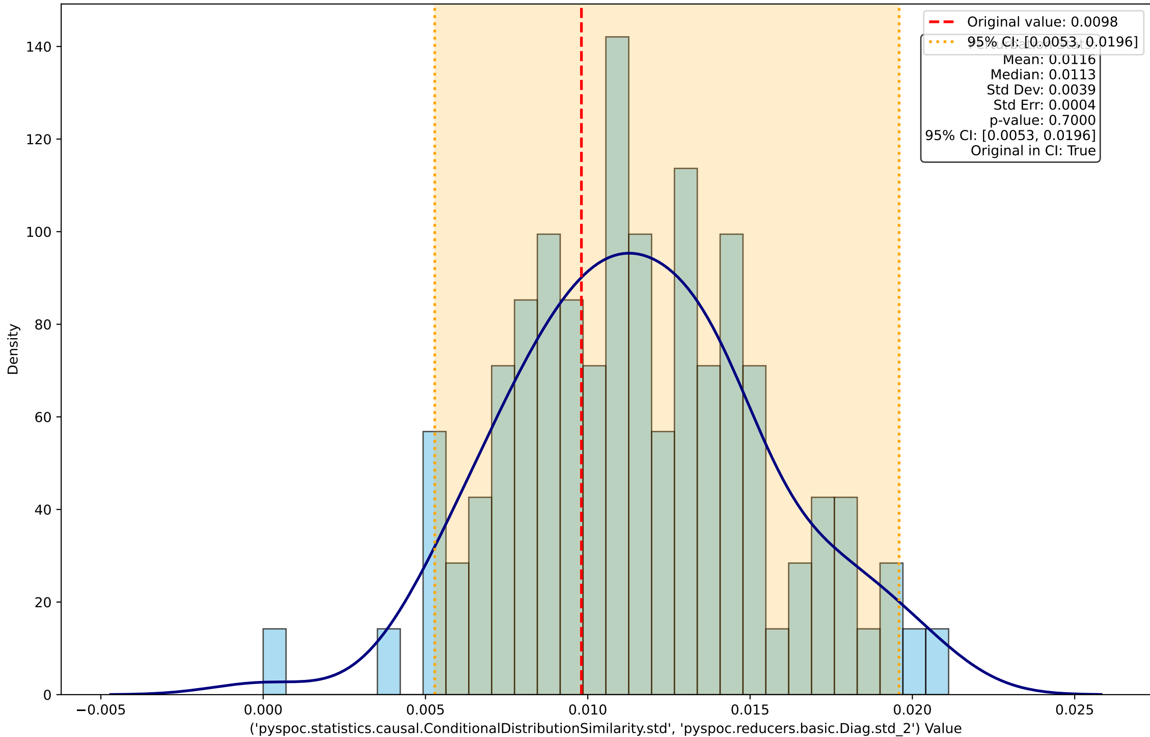
Perturbation Distribution for ('pypoc.statistics.causal.ConditionalDistributionSimilarity.std', 'pypoc.reducers.basic.Diag.std_2')
