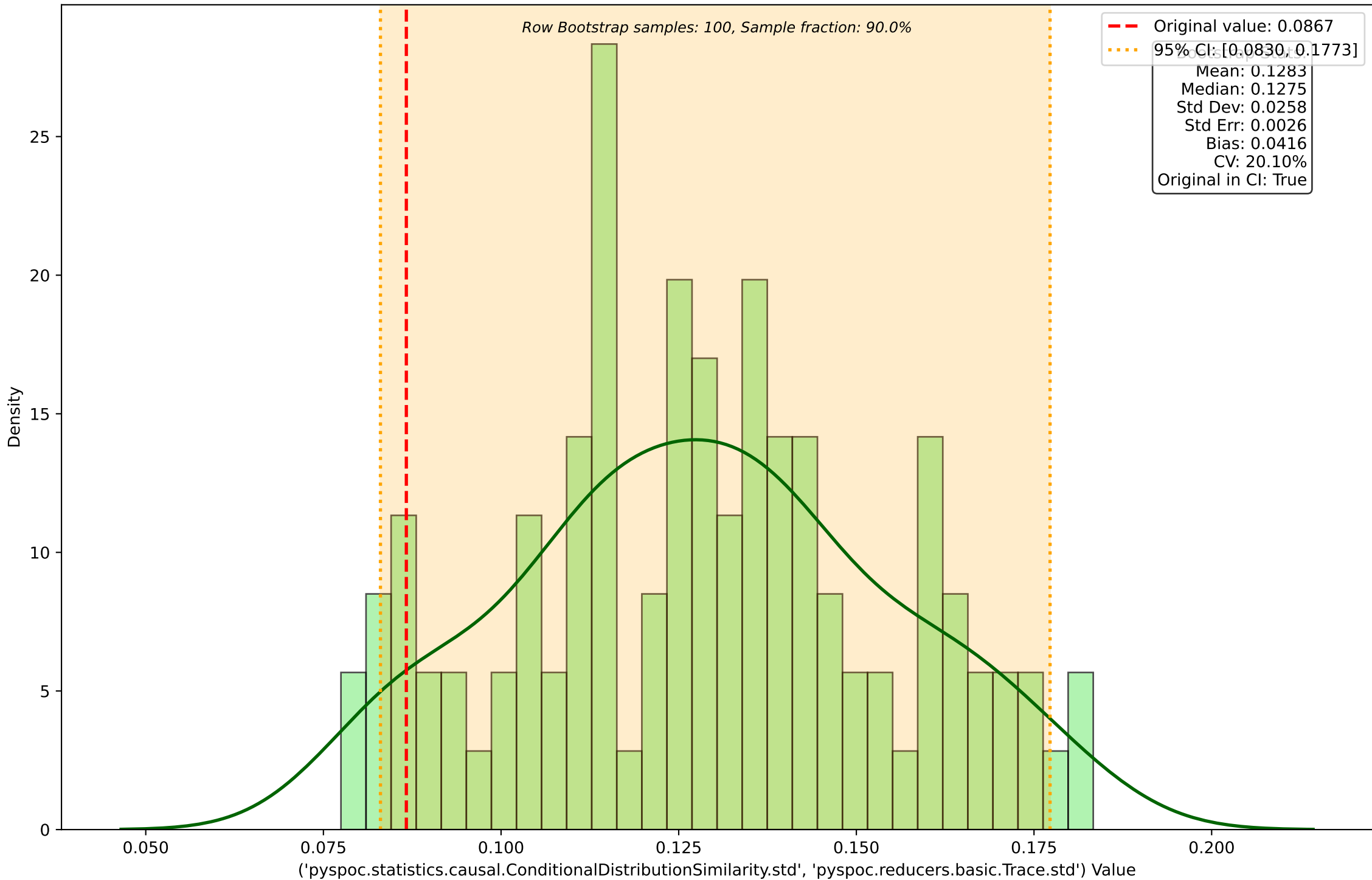
Row Bootstrap Distribution for ('pypoc.statistics.causal.ConditionalDistributionSimilarity.std', 'pypoc.reducers.basic.Trace.std')
