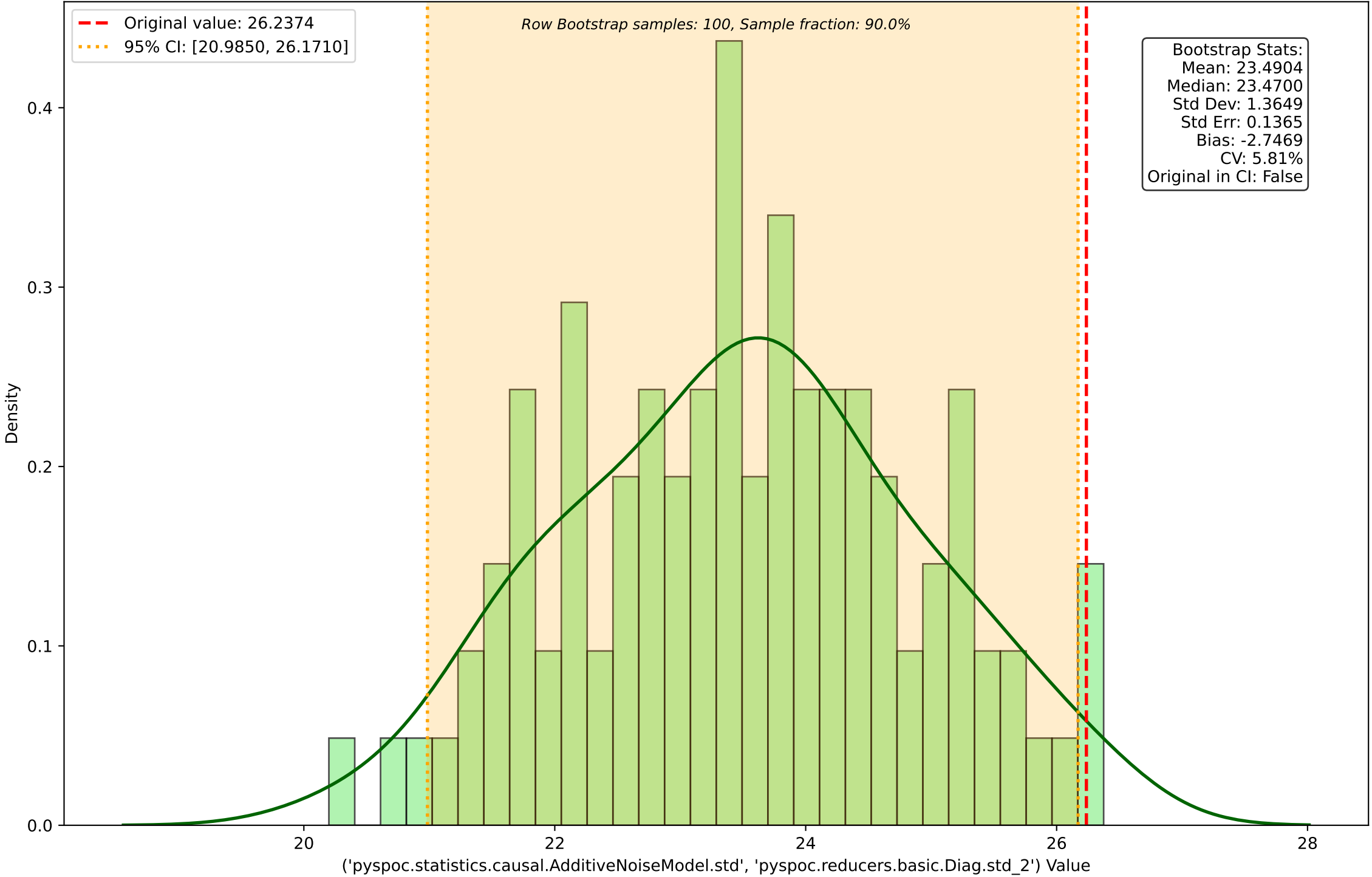
Row Bootstrap Distribution for ('pyspoc.statistics.causal.AdditiveNoiseModel.std', 'pyspoc.reducers.basic.Diag.std_2')
