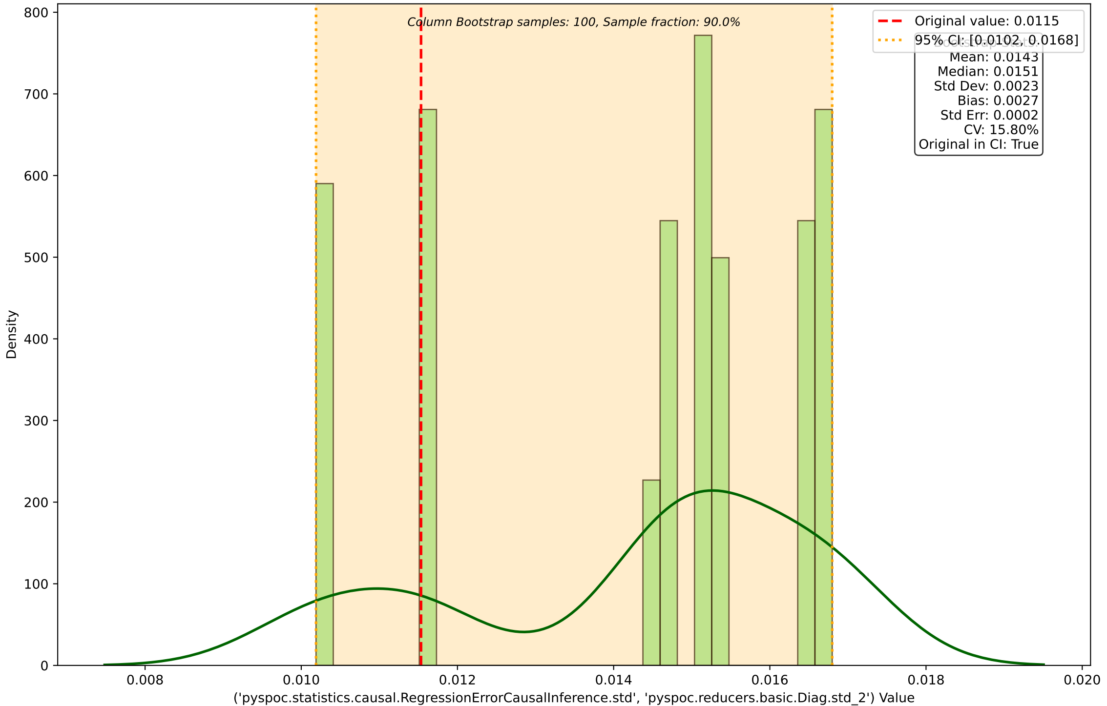
Column Bootstrap Distribution for ('pypoc.statistics.causal.RegressionErrorCausalInference.std', 'pypoc.reducers.basic.Diag.std_2')
