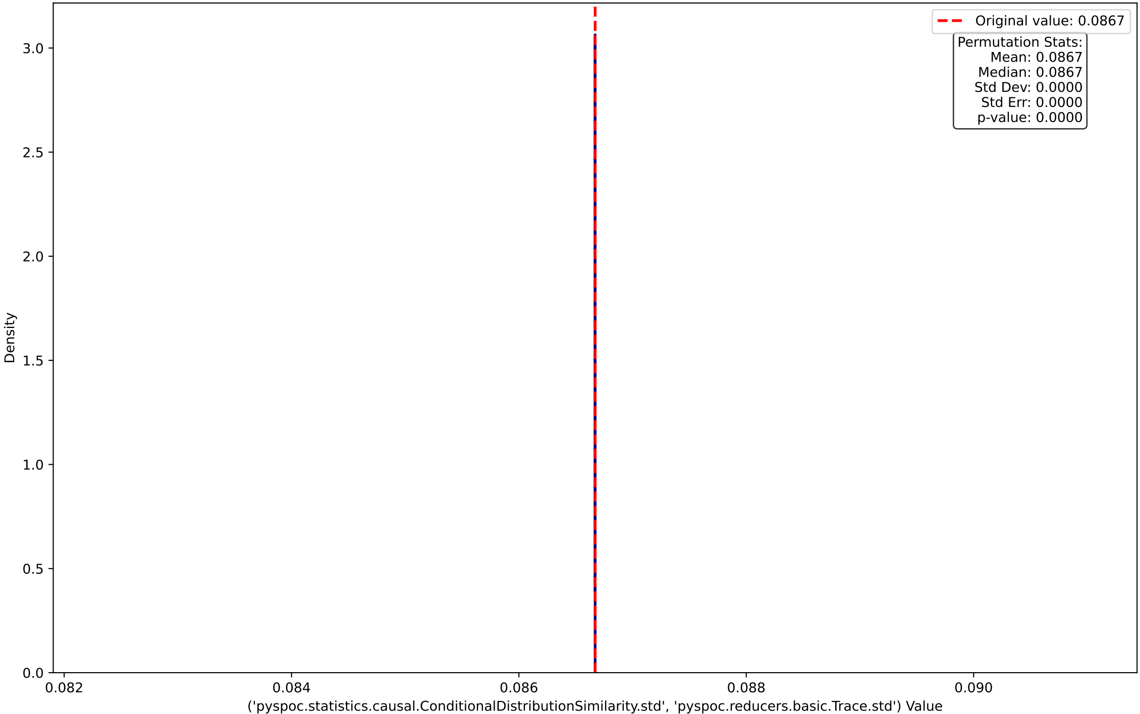
1e16 Permutation Distribution for ('pyspoc.statistics.causal.ConditionalDistributionSimilarity.std', 'pyspoc.reducers.basic.Trace.std')
