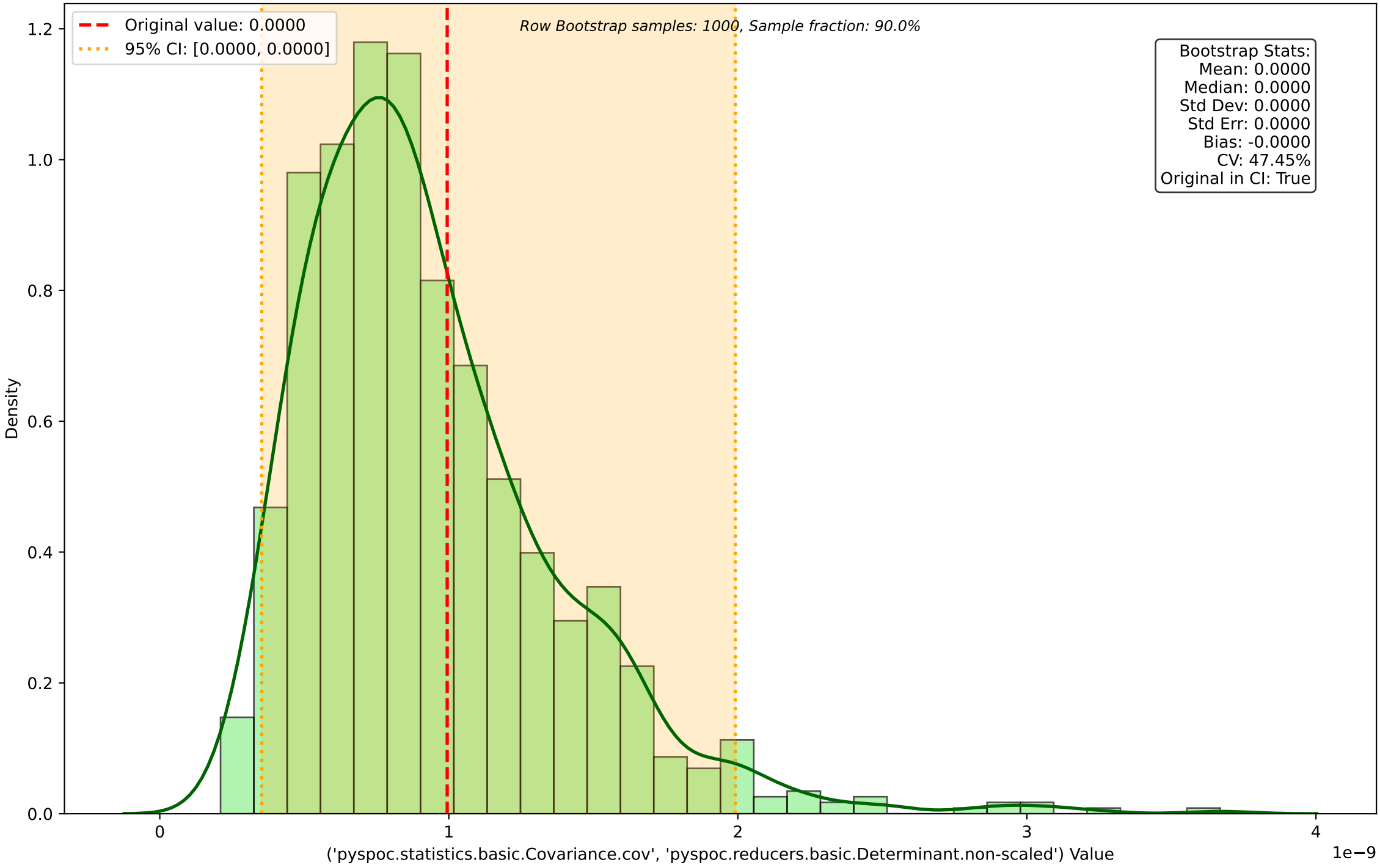
Row Bootstrap Distribution for ('pyspoc.statistics.basic.Covariance.cov', 'pyspoc.reducers.basic.Determinant.non-scaled')
