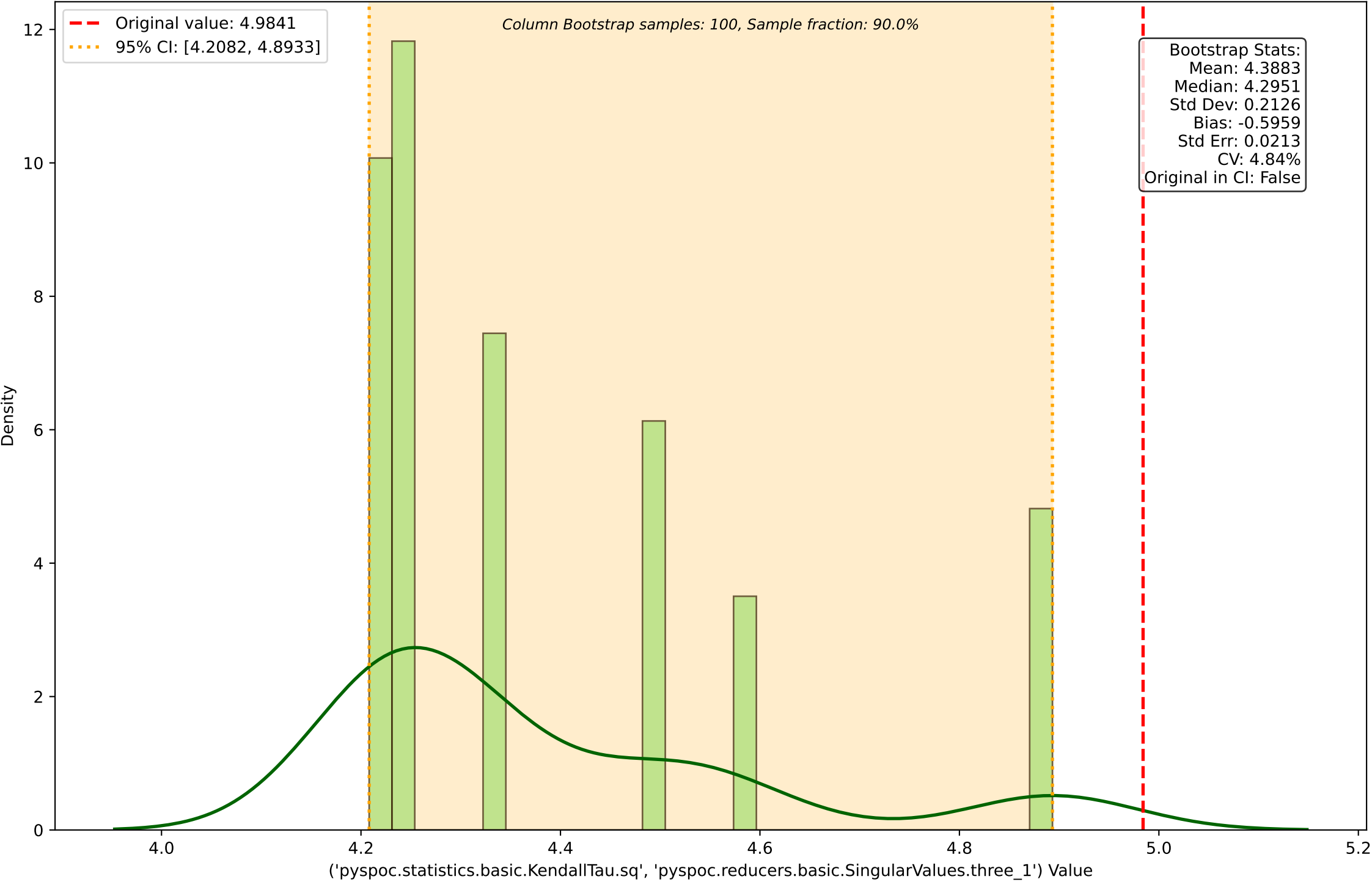
Column Bootstrap Distribution for ('pyspoc.statistics.basic.KendallTau.sq', 'pyspoc.reducers.basic.SingularValues.three_1')
