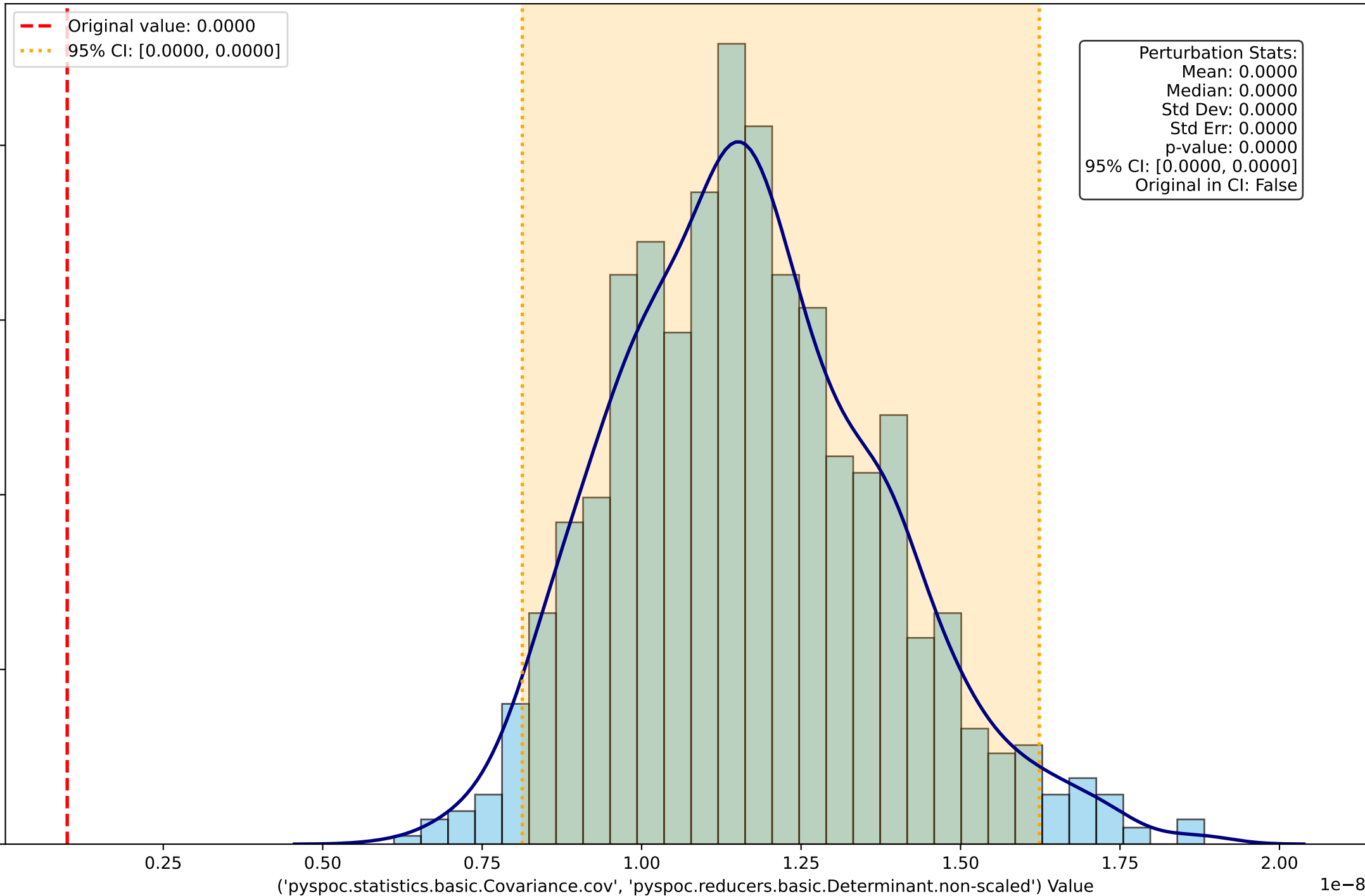
Perturbation Distribution for ('pyspoc.statistics.basic.Covariance.cov', 'pyspoc.reducers.basic.Determinant.non-scaled')
