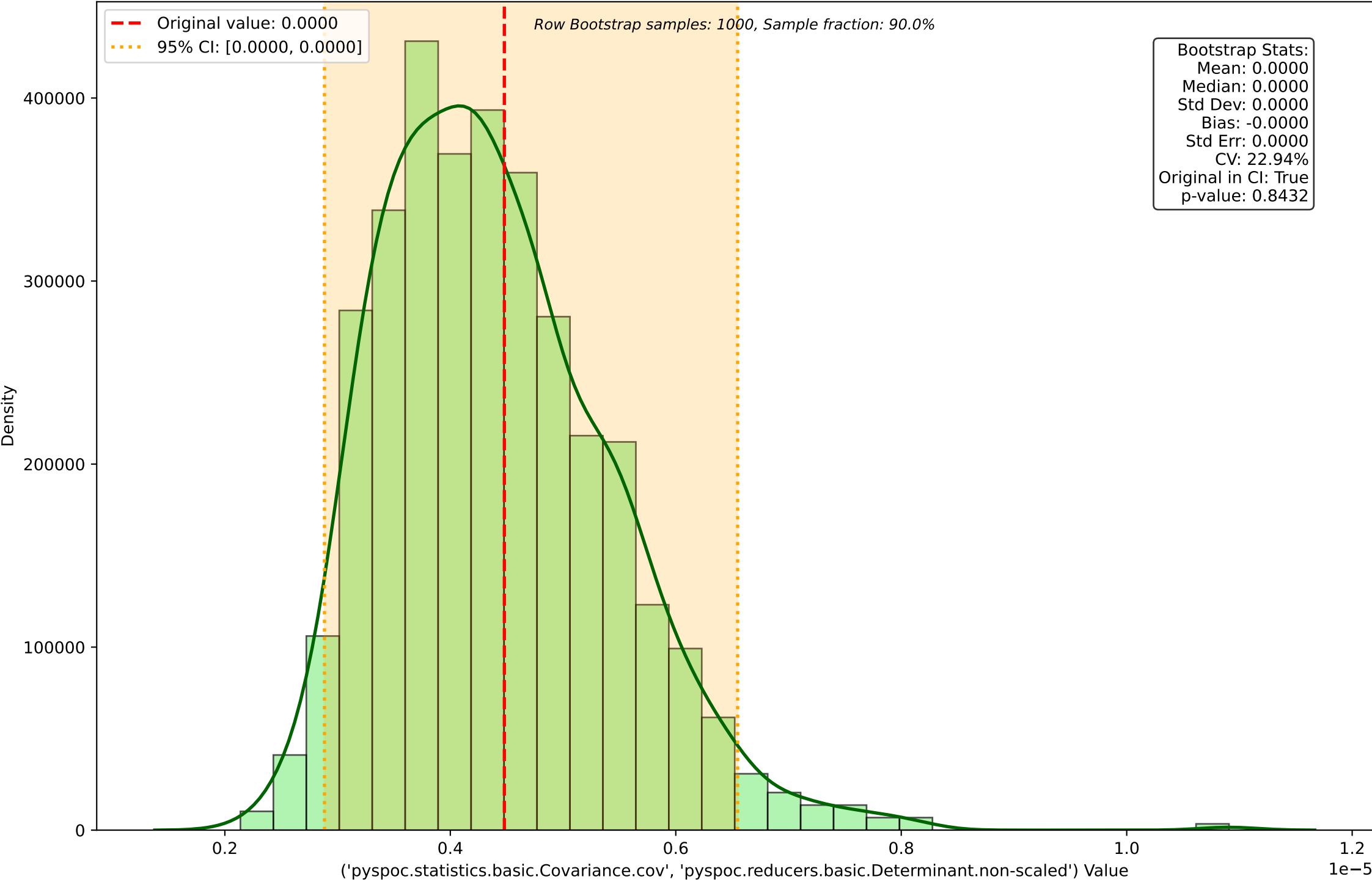
Row Bootstrap Distribution for ('pyspoc.statistics.basic.Covariance.cov', 'pyspoc.reducers.basic.Determinant.non-scaled')
