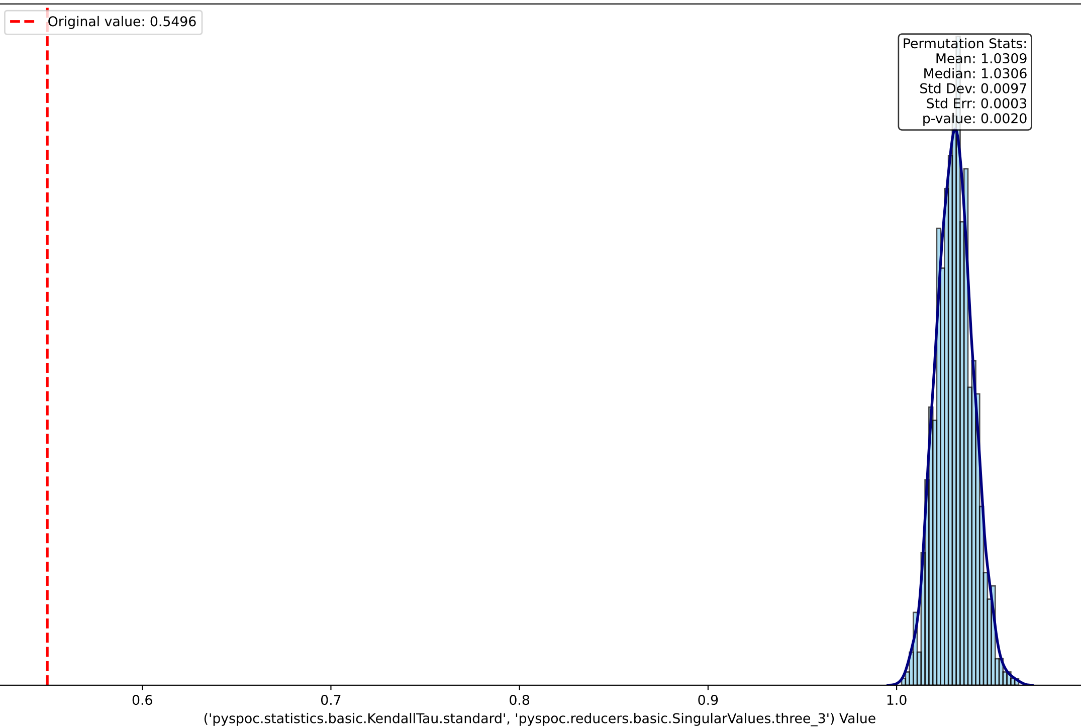
Permutation Distribution for ('pyspoc.statistics.basic.KendallTau.standard', 'pyspoc.reducers.basic.SingularValues.three_3')
