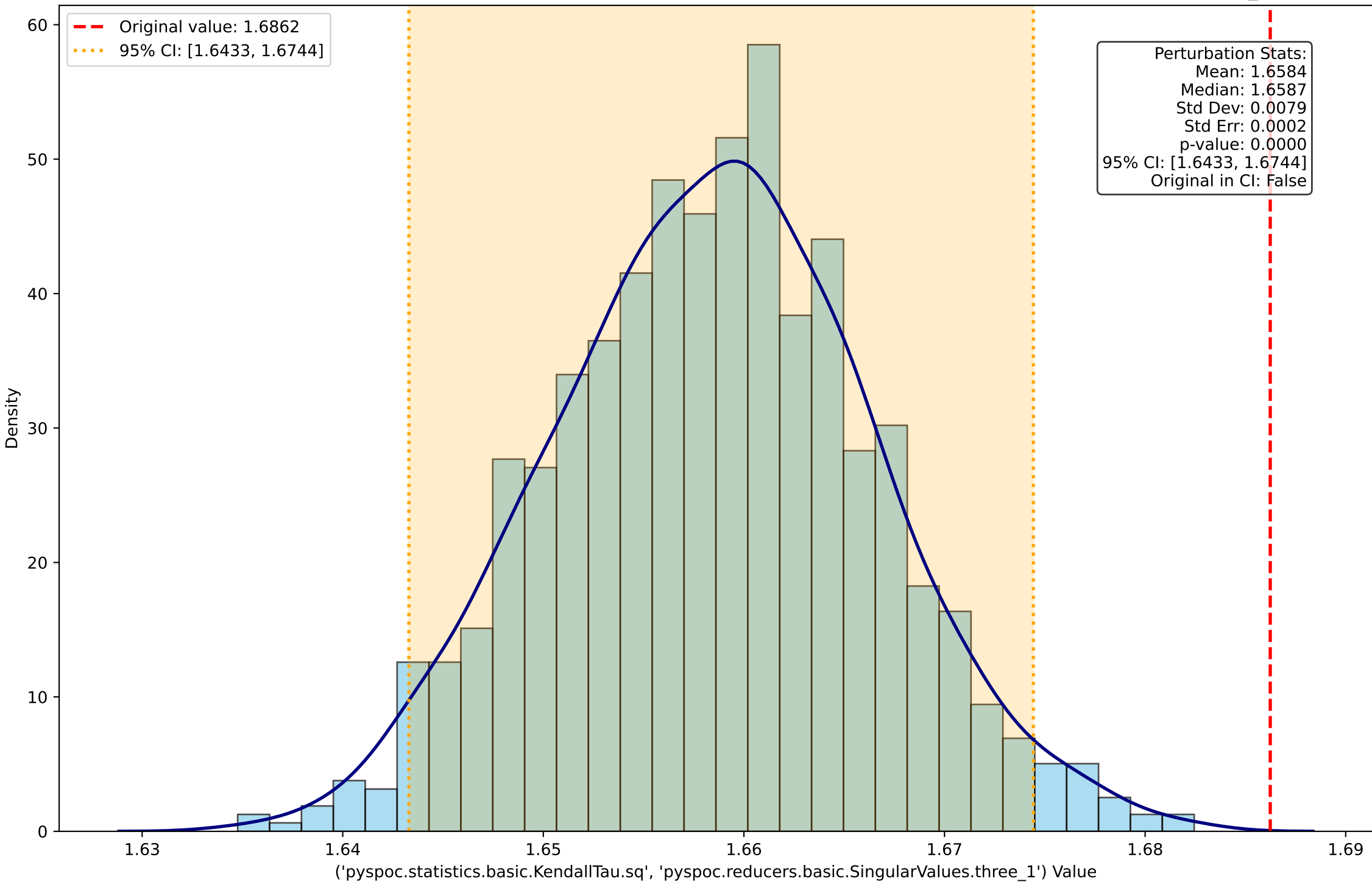
Perturbation Distribution for ('pyspoc.statistics.basic.KendallTau.sq', 'pyspoc.reducers.basic.SingularValues.three_1')
