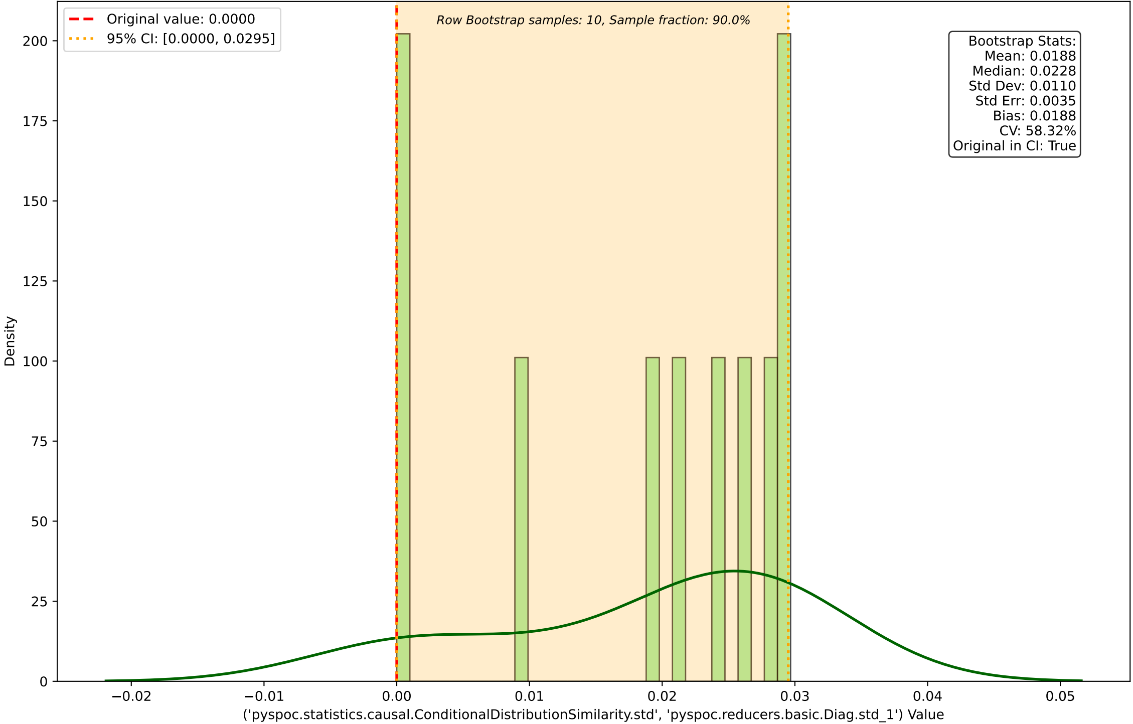
Row Bootstrap Distribution for ('pyspoc.statistics.causal.ConditionalDistributionSimilarity.std', 'pyspoc.reducers.basic.Diag.std_1')
