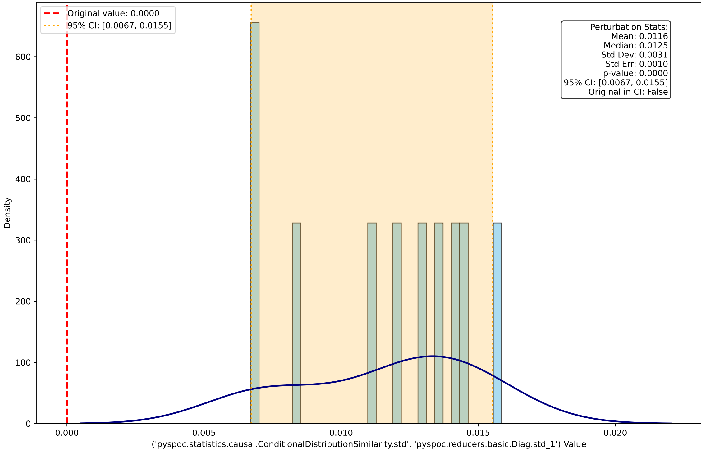
Perturbation Distribution for ('pyspoc.statistics.causal.ConditionalDistributionSimilarity.std', 'pyspoc.reducers.basic.Diag.std_1')
