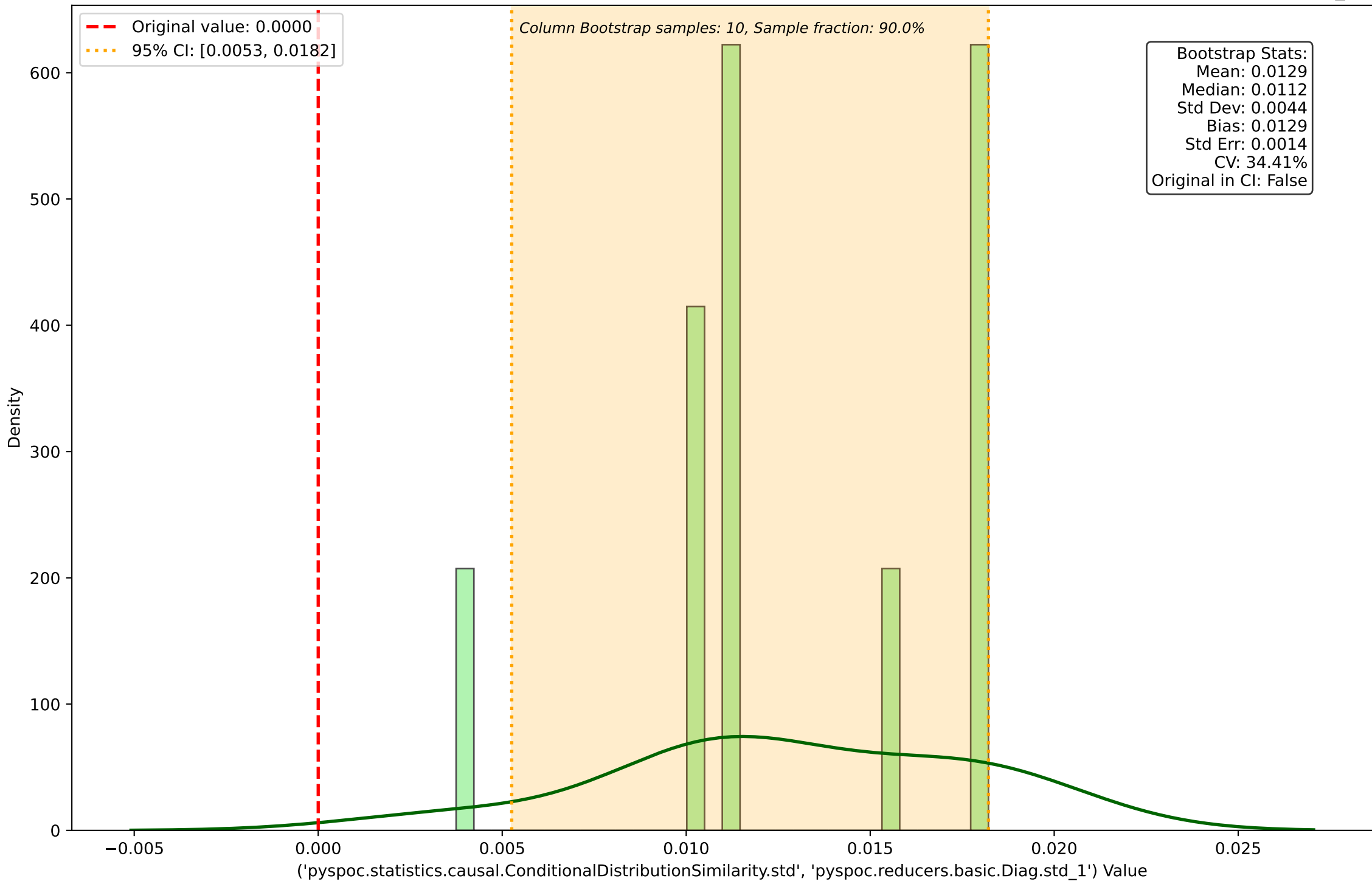
Column Bootstrap Distribution for ('pyspoc.statistics.causal.ConditionalDistributionSimilarity.std', 'pyspoc.reducers.basic.Diag.std_1')
