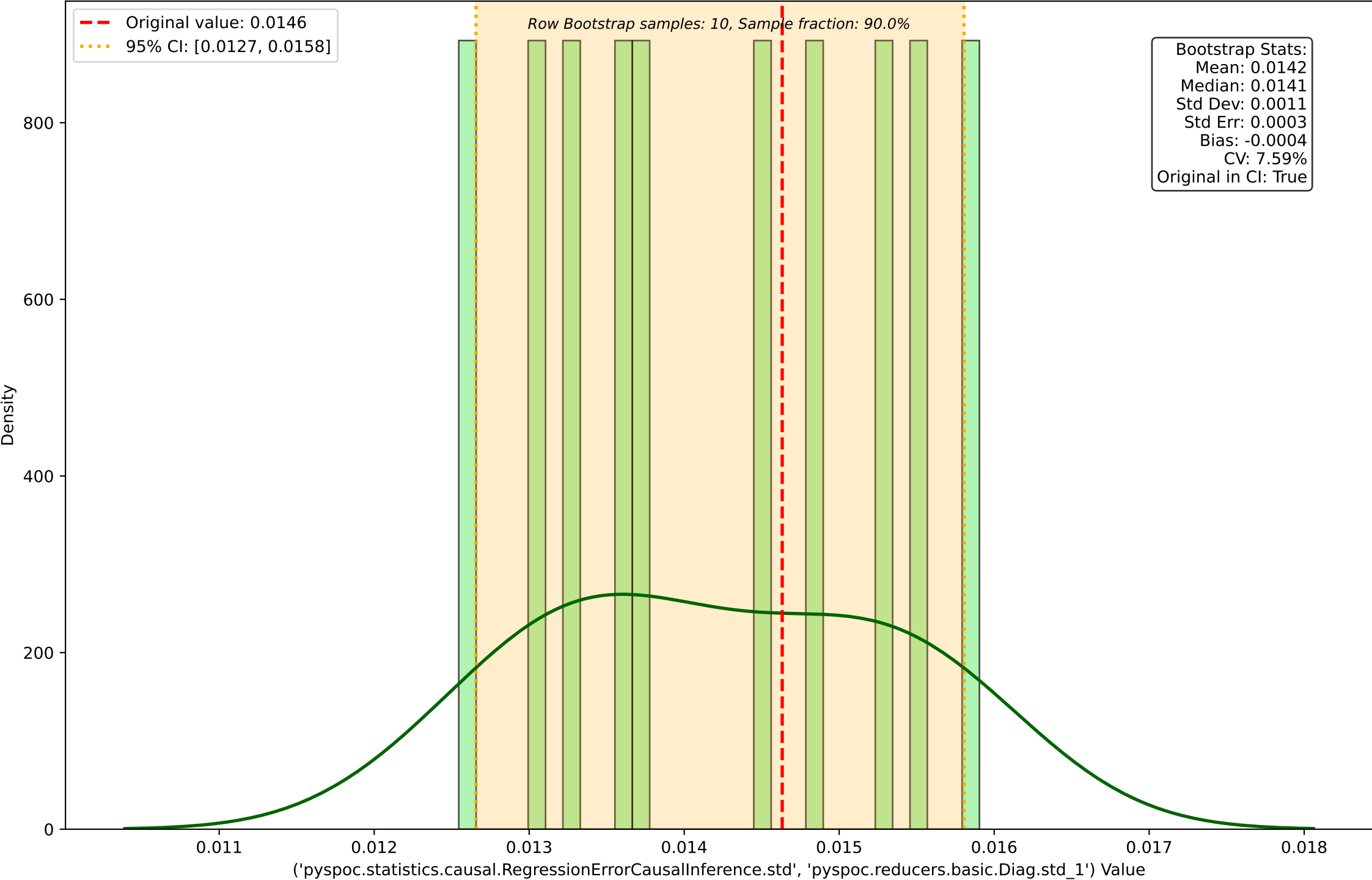
Row Bootstrap Distribution for ('pyspoc.statistics.causal.RegressionErrorCausalInference.std', 'pyspoc.reducers.basic.Diag.std_1')
