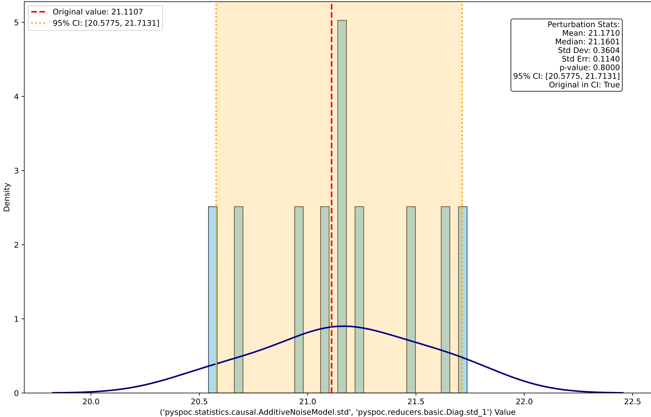
Perturbation Distribution for ('pyspoc.statistics.causal.AdditiveNoiseModel.std', 'pyspoc.reducers.basic.Diag.std_1')
