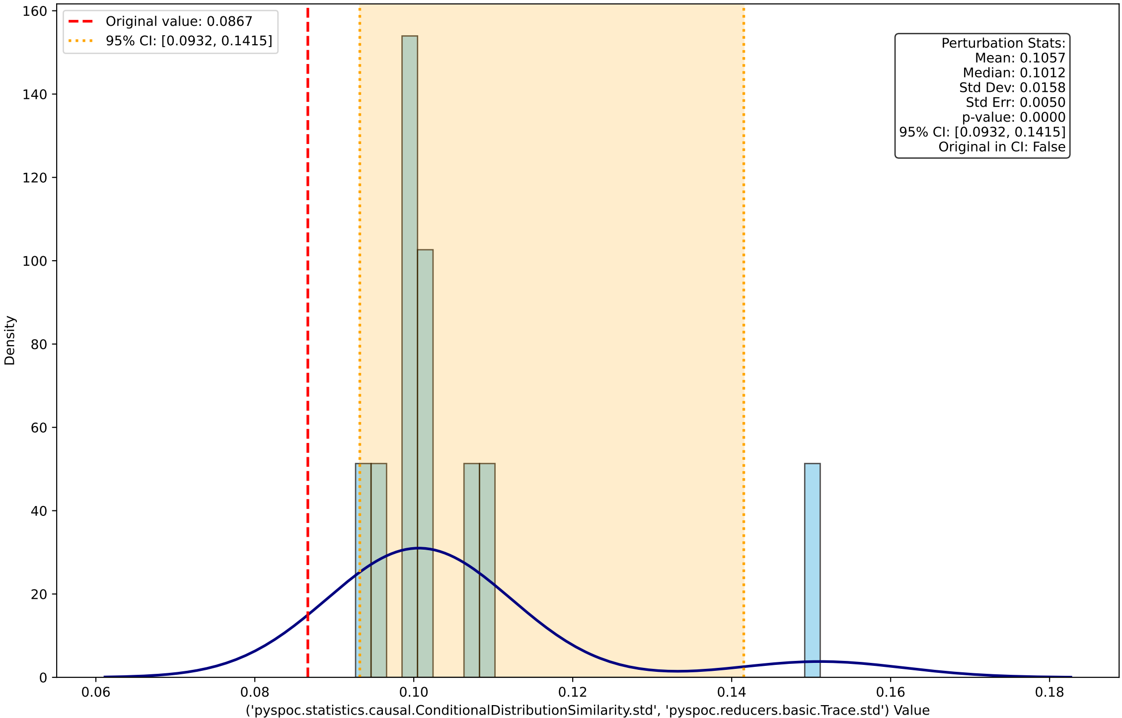
Perturbation Distribution for ('pyspoc.statistics.causal.ConditionalDistributionSimilarity.std', 'pyspoc.reducers.basic.Trace.std')
