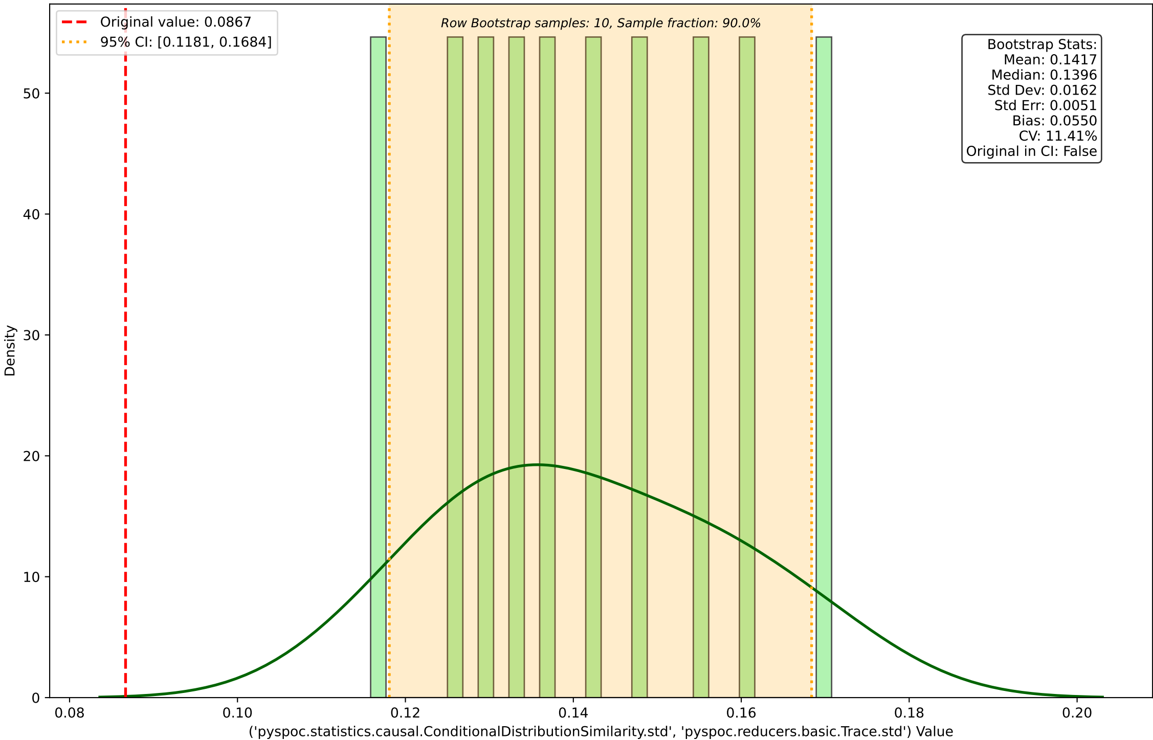
Row Bootstrap Distribution for ('pyspoc.statistics.causal.ConditionalDistributionSimilarity.std', 'pyspoc.reducers.basic.Trace.std')
