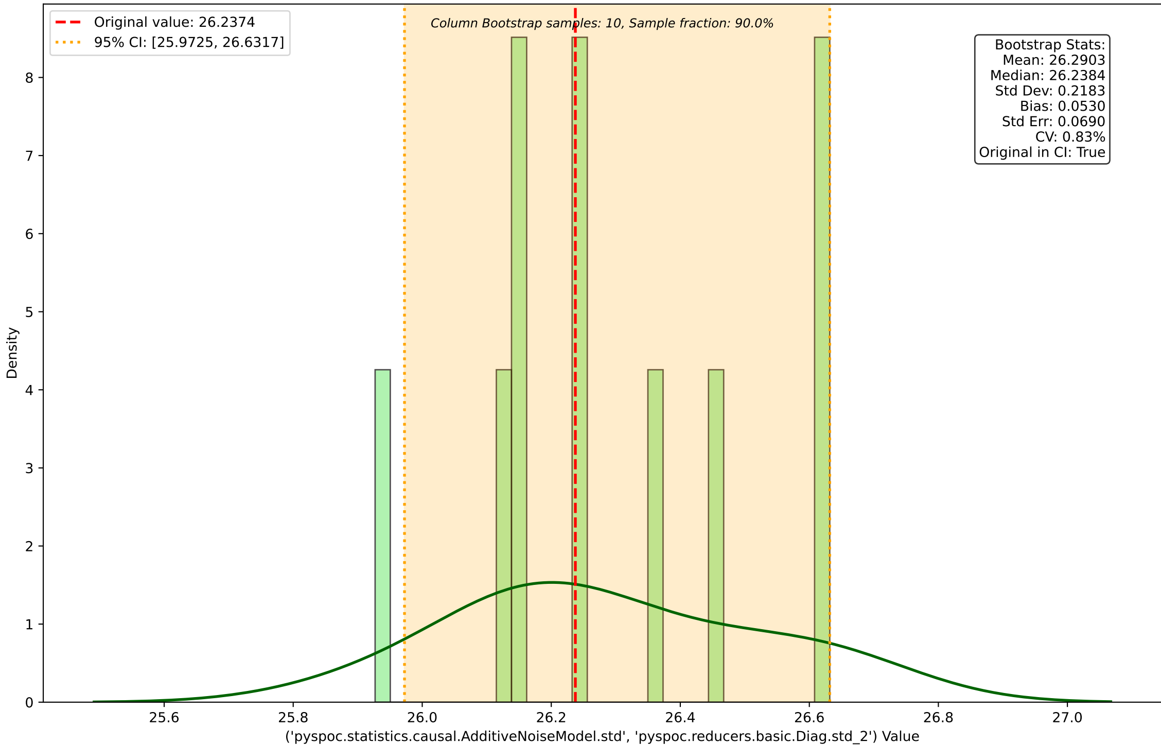
Column Bootstrap Distribution for ('pyspoc.statistics.causal.AdditiveNoiseModel.std', 'pyspoc.reducers.basic.Diag.std_2')
