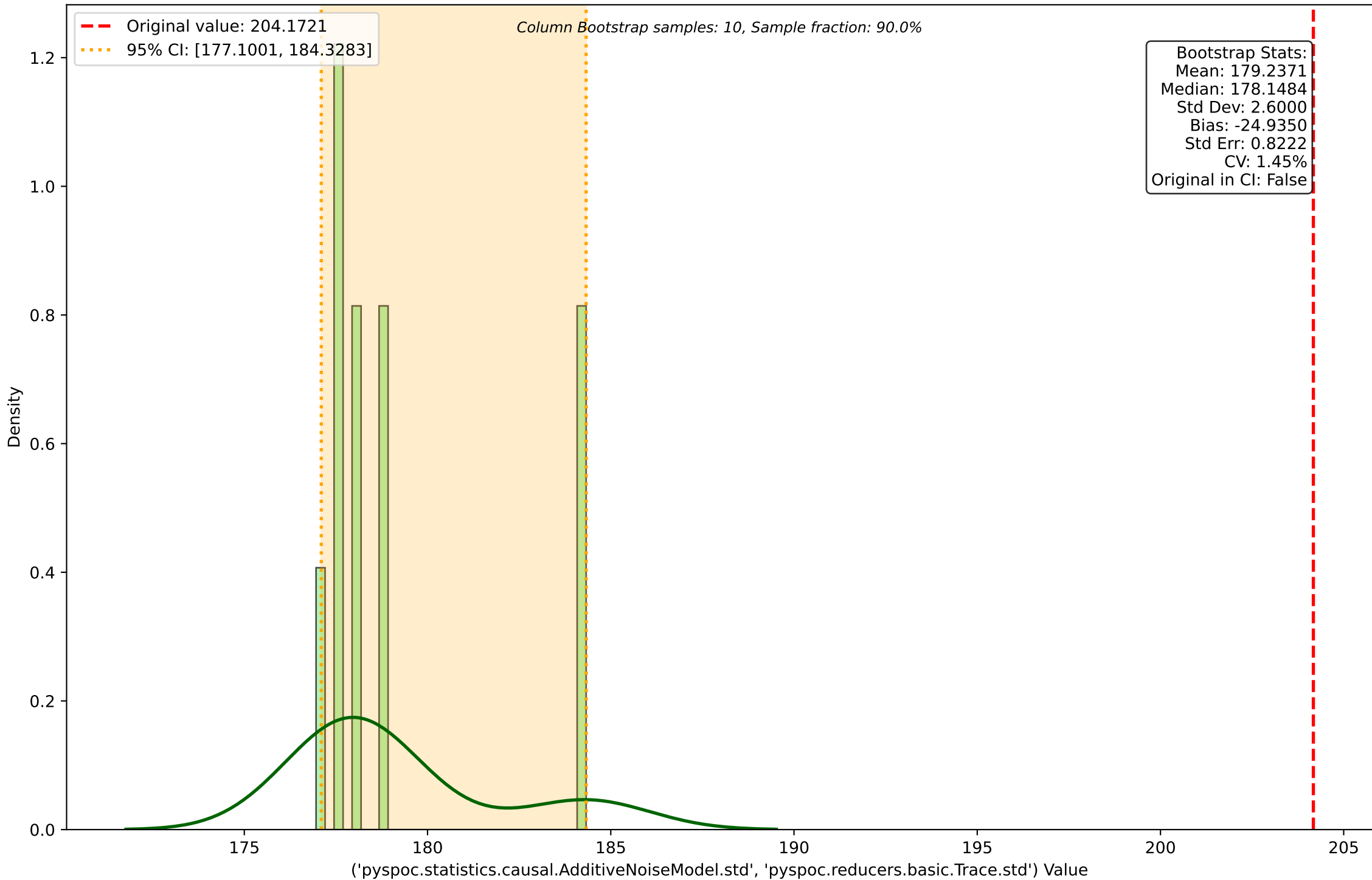
Column Bootstrap Distribution for ('pyspoc.statistics.causal.AdditiveNoiseModel.std', 'pyspoc.reducers.basic.Trace.std')
