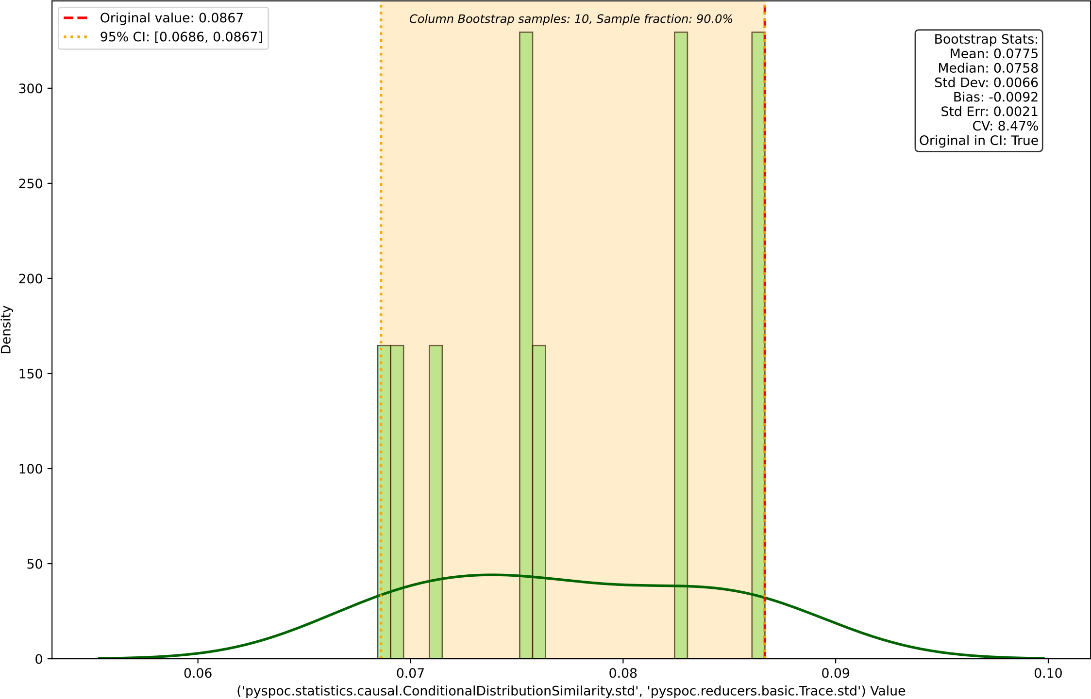
Column Bootstrap Distribution for ('pyspoc.statistics.causal.ConditionalDistributionSimilarity.std', 'pyspoc.reducers.basic.Trace.std')
