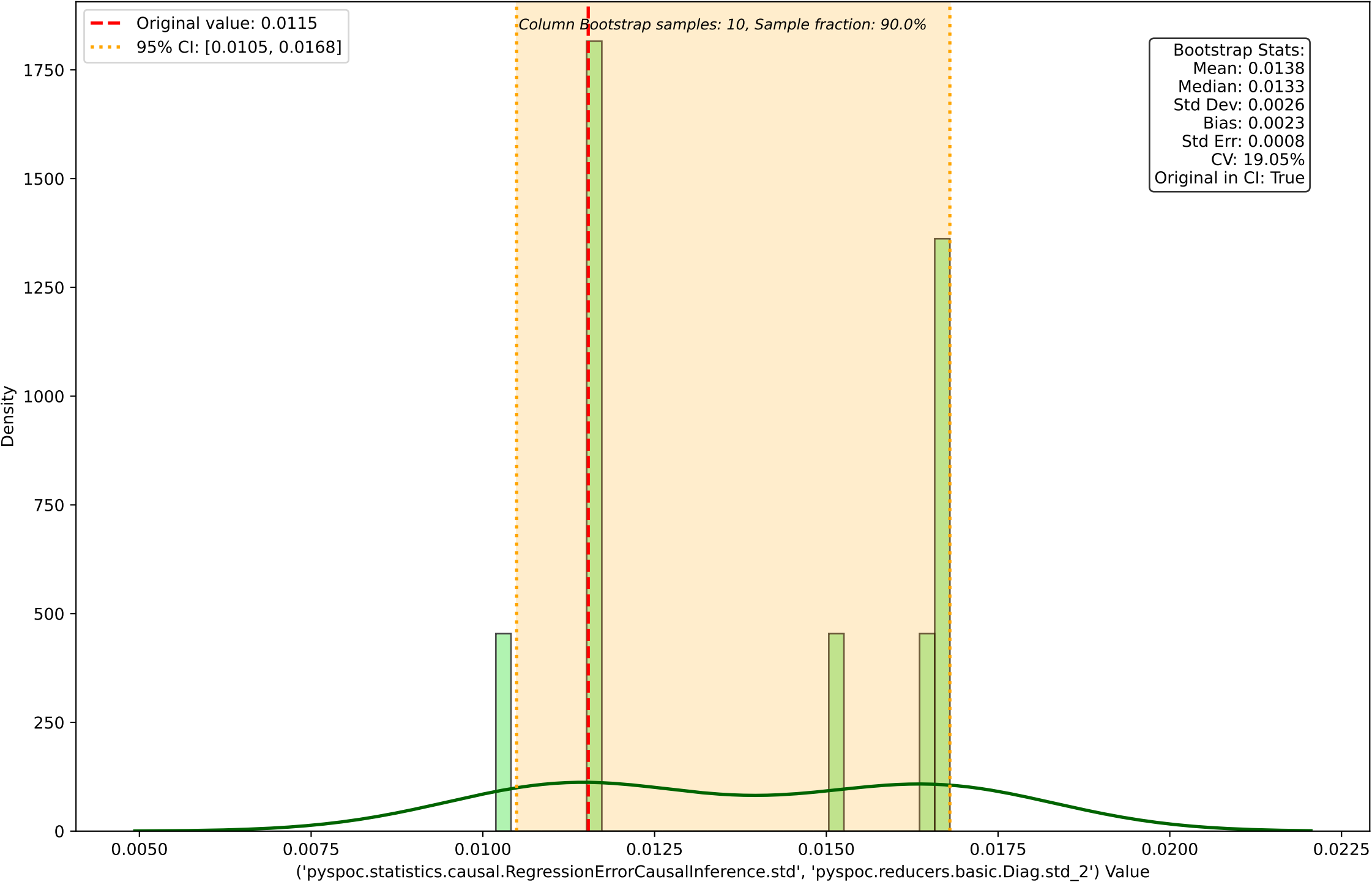
Column Bootstrap Distribution for ('pyspoc.statistics.causal.RegressionErrorCausalInference.std', 'pyspoc.reducers.basic.Diag.std_2')
