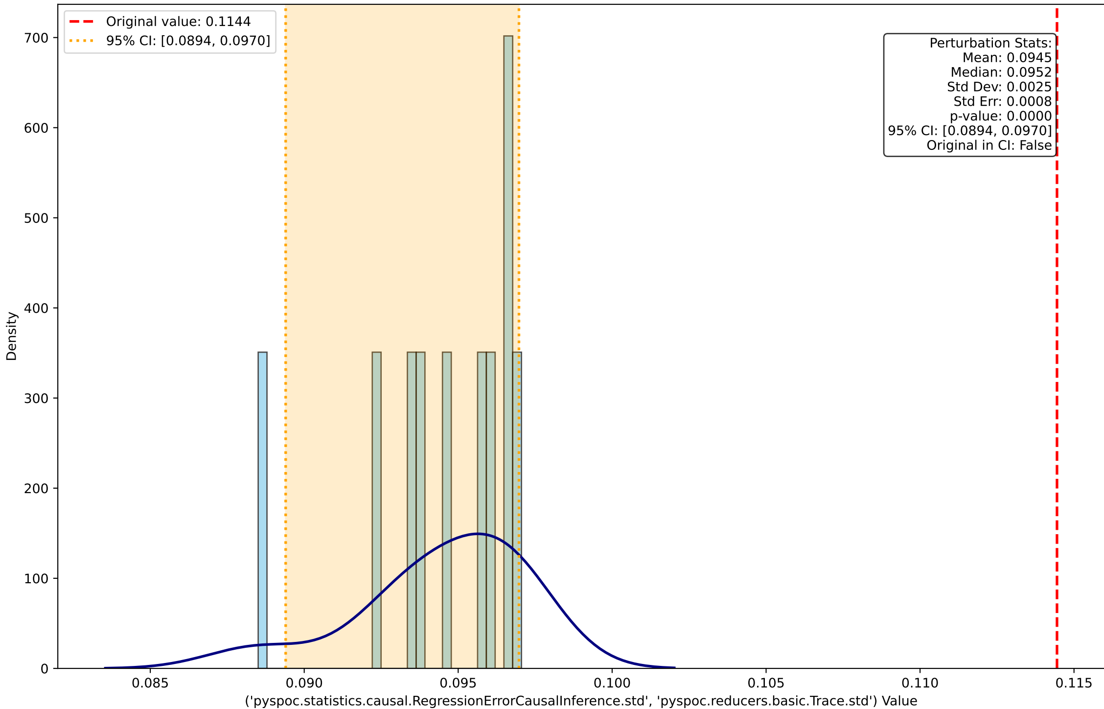
Perturbation Distribution for ('pyspoc.statistics.causal.RegressionErrorCausalInference.std', 'pyspoc.reducers.basic.Trace.std')
