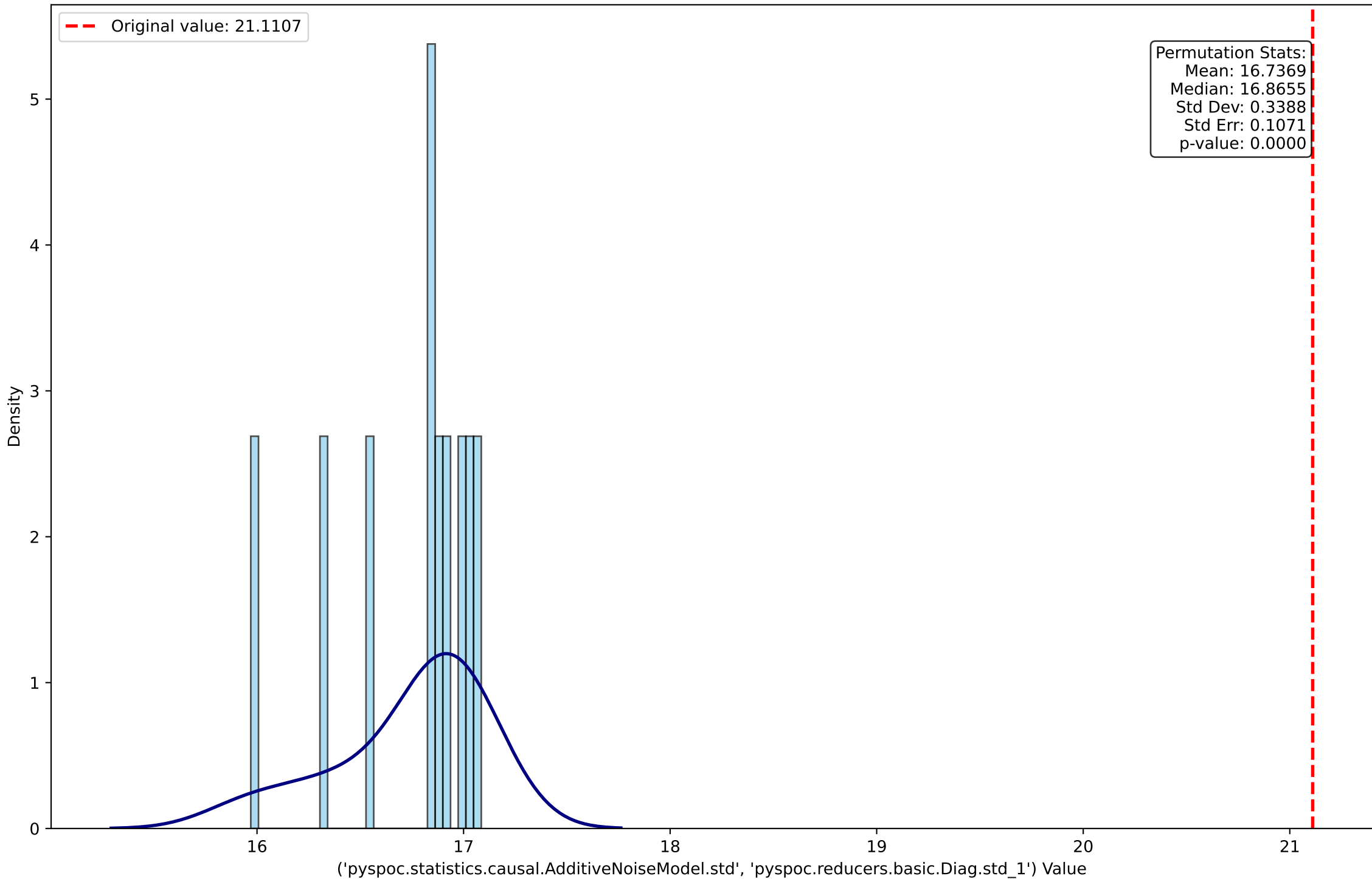
Permutation Distribution for ('pyspoc.statistics.causal.AdditiveNoiseModel.std', 'pyspoc.reducers.basic.Diag.std_1')
