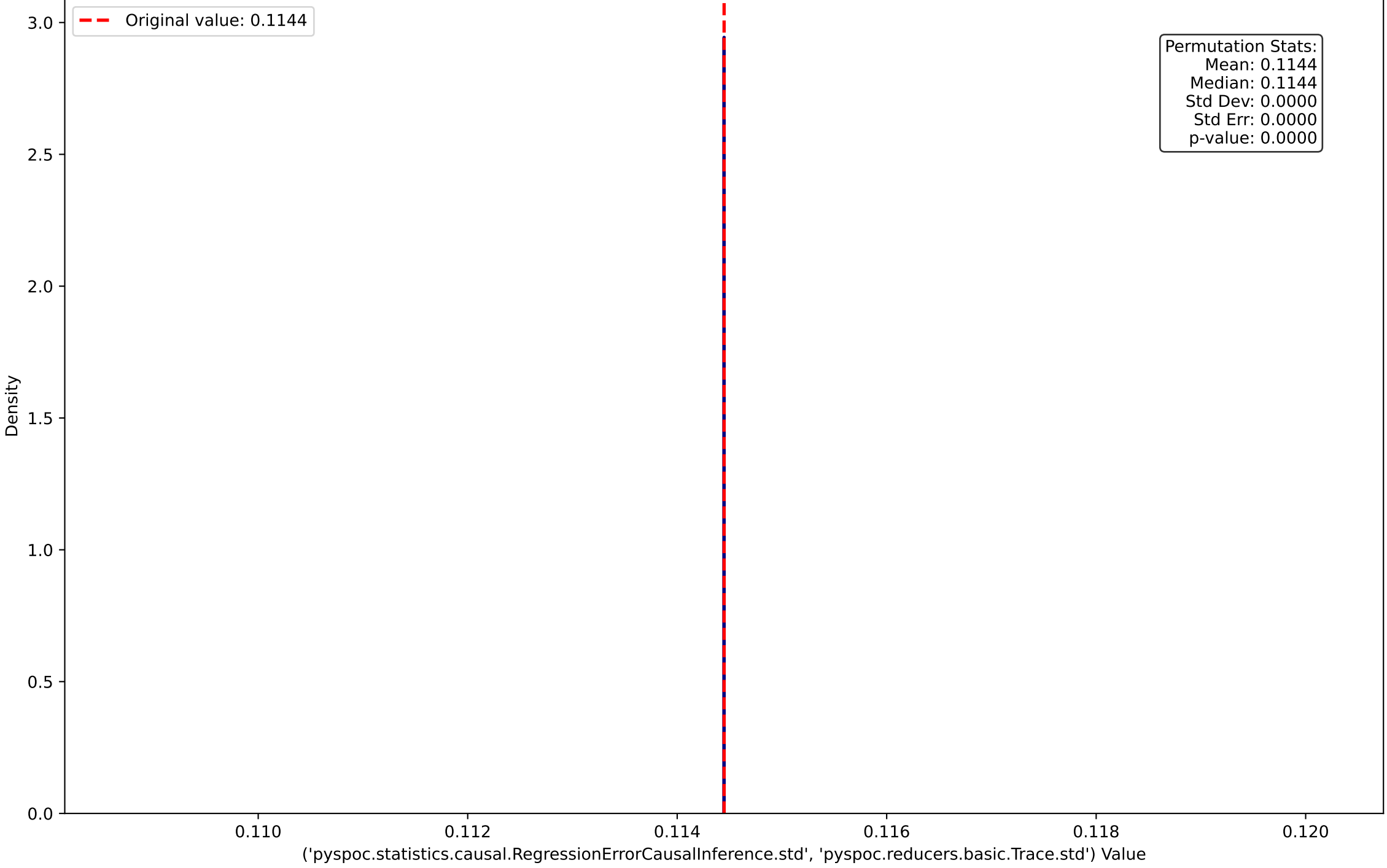
1e16 Permutation Distribution for ('pyspoc.statistics.causal.RegressionErrorCausalInference.std', 'pyspoc.reducers.basic.Trace.std')
