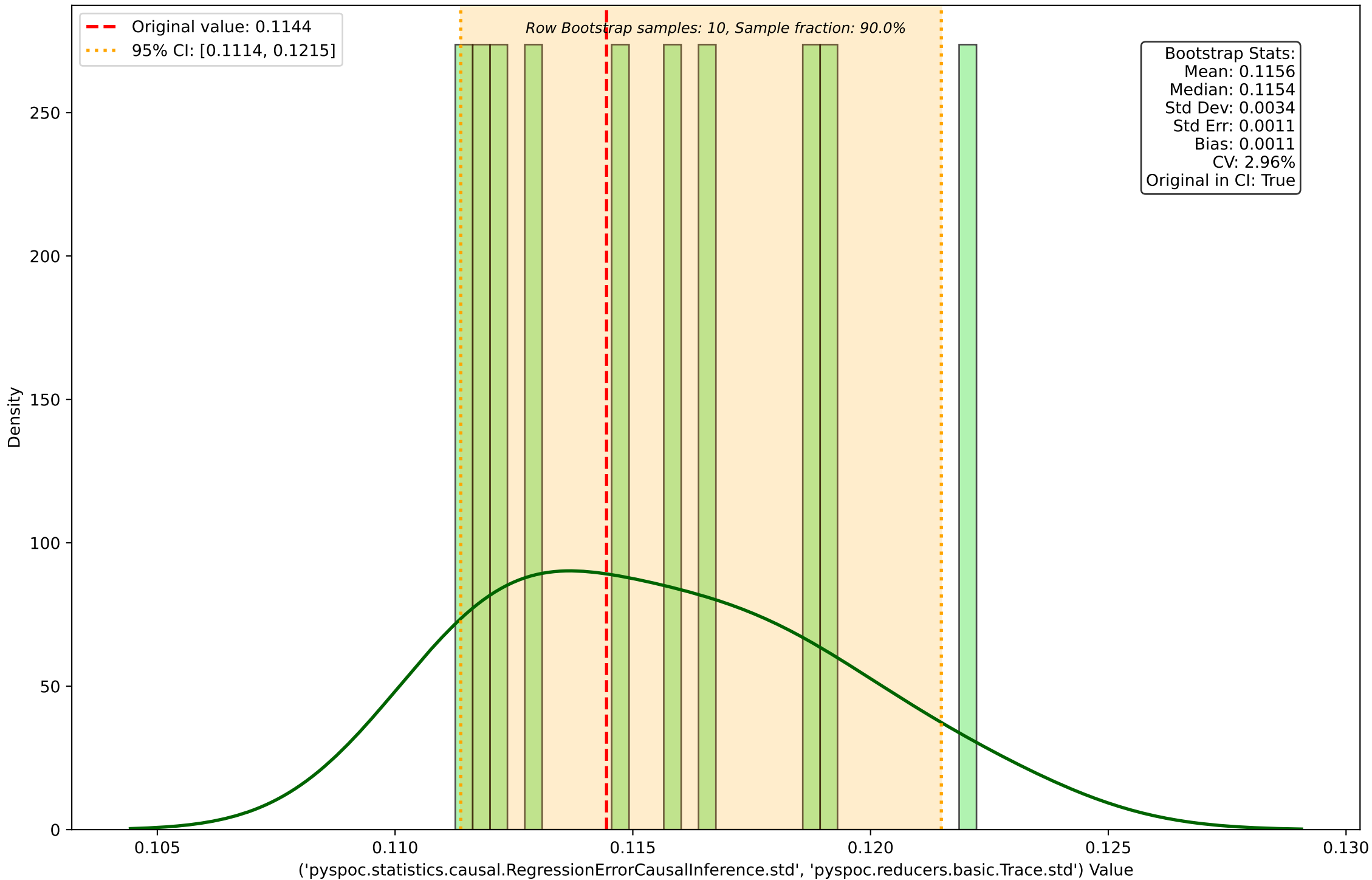
Row Bootstrap Distribution for ('pyspoc.statistics.causal.RegressionErrorCausalInference.std', 'pyspoc.reducers.basic.Trace.std')
