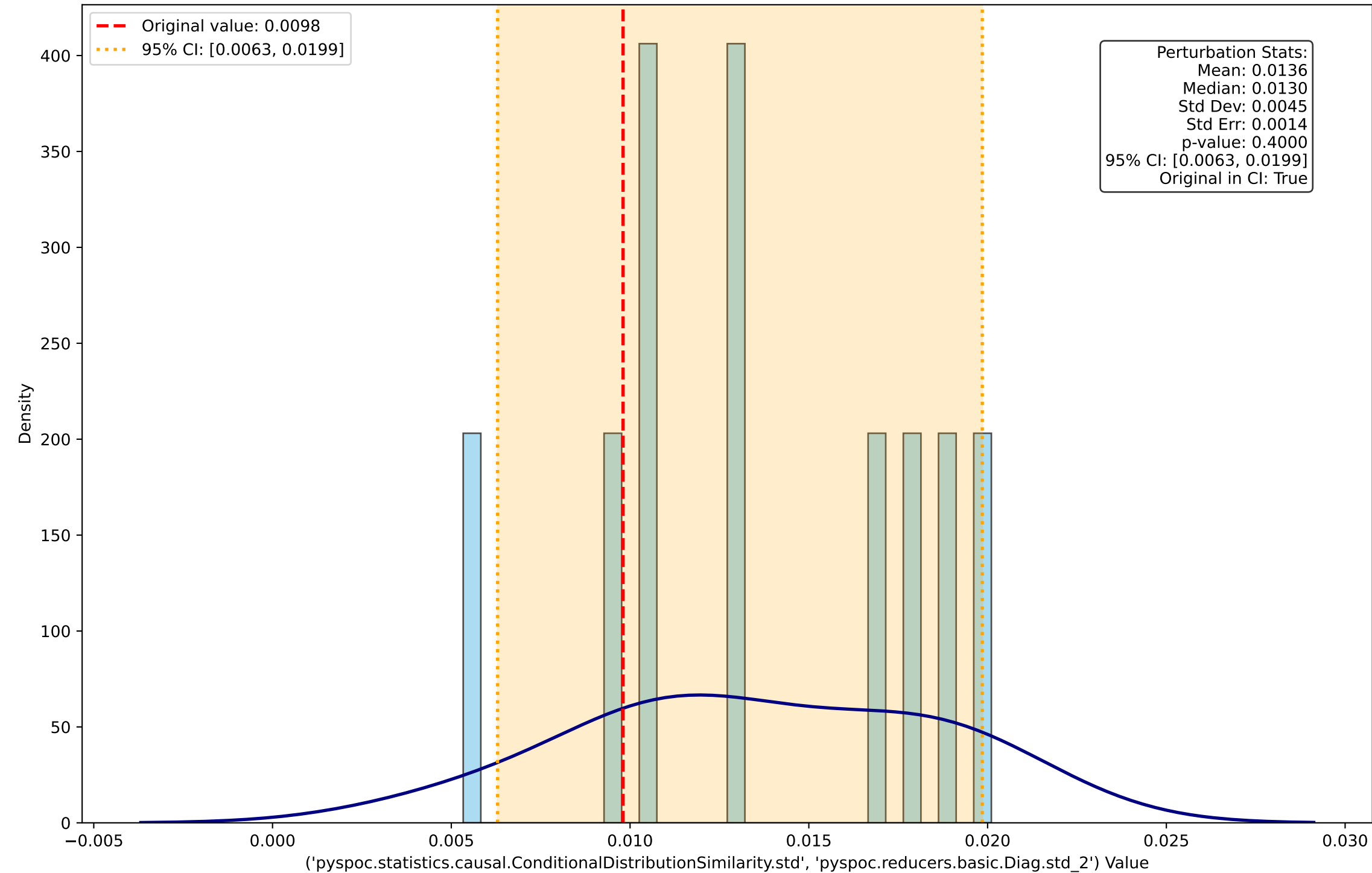
Perturbation Distribution for ('pyspoc.statistics.causal.ConditionalDistributionSimilarity.std', 'pyspoc.reducers.basic.Diag.std_2')
