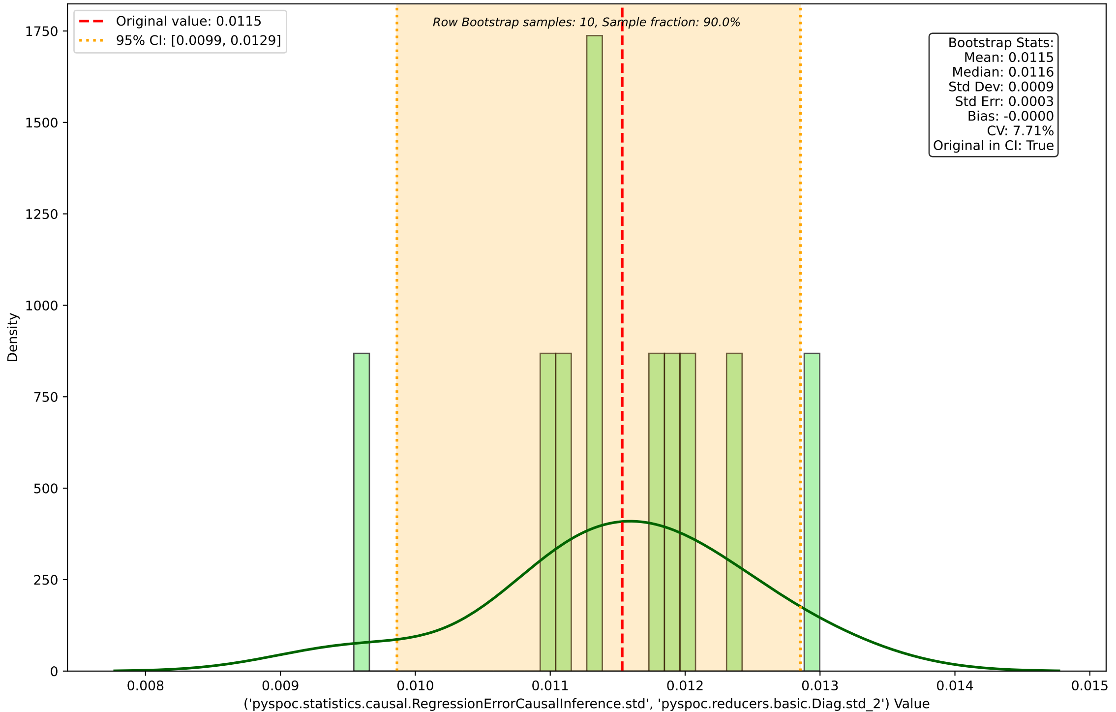
Row Bootstrap Distribution for ('pyspoc.statistics.causal.RegressionErrorCausalInference.std', 'pyspoc.reducers.basic.Diag.std_2')
