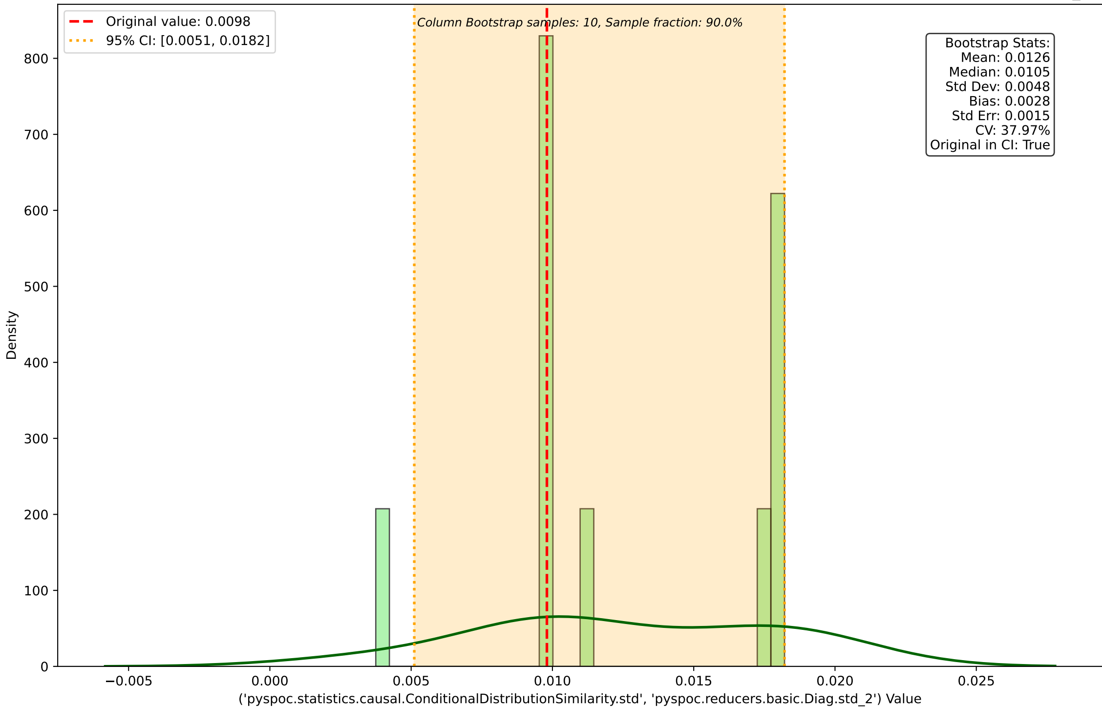
Column Bootstrap Distribution for ('pypoc.statistics.causal.ConditionalDistributionSimilarity.std', 'pypoc.reducers.basic.Diag.std_2')
