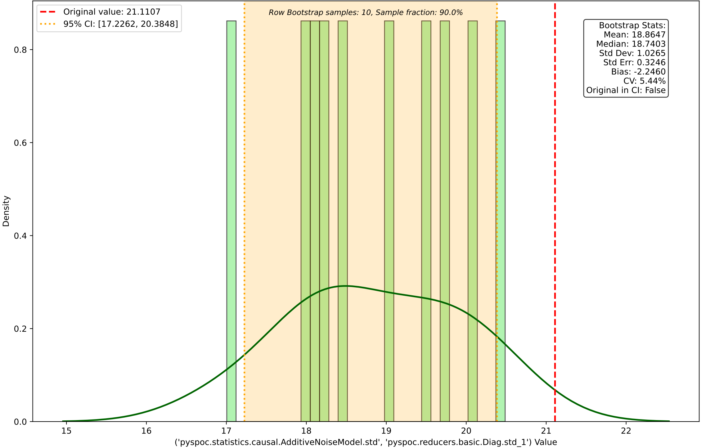
Row Bootstrap Distribution for ('pyspoc.statistics.causal.AdditiveNoiseModel.std', 'pyspoc.reducers.basic.Diag.std_1')
