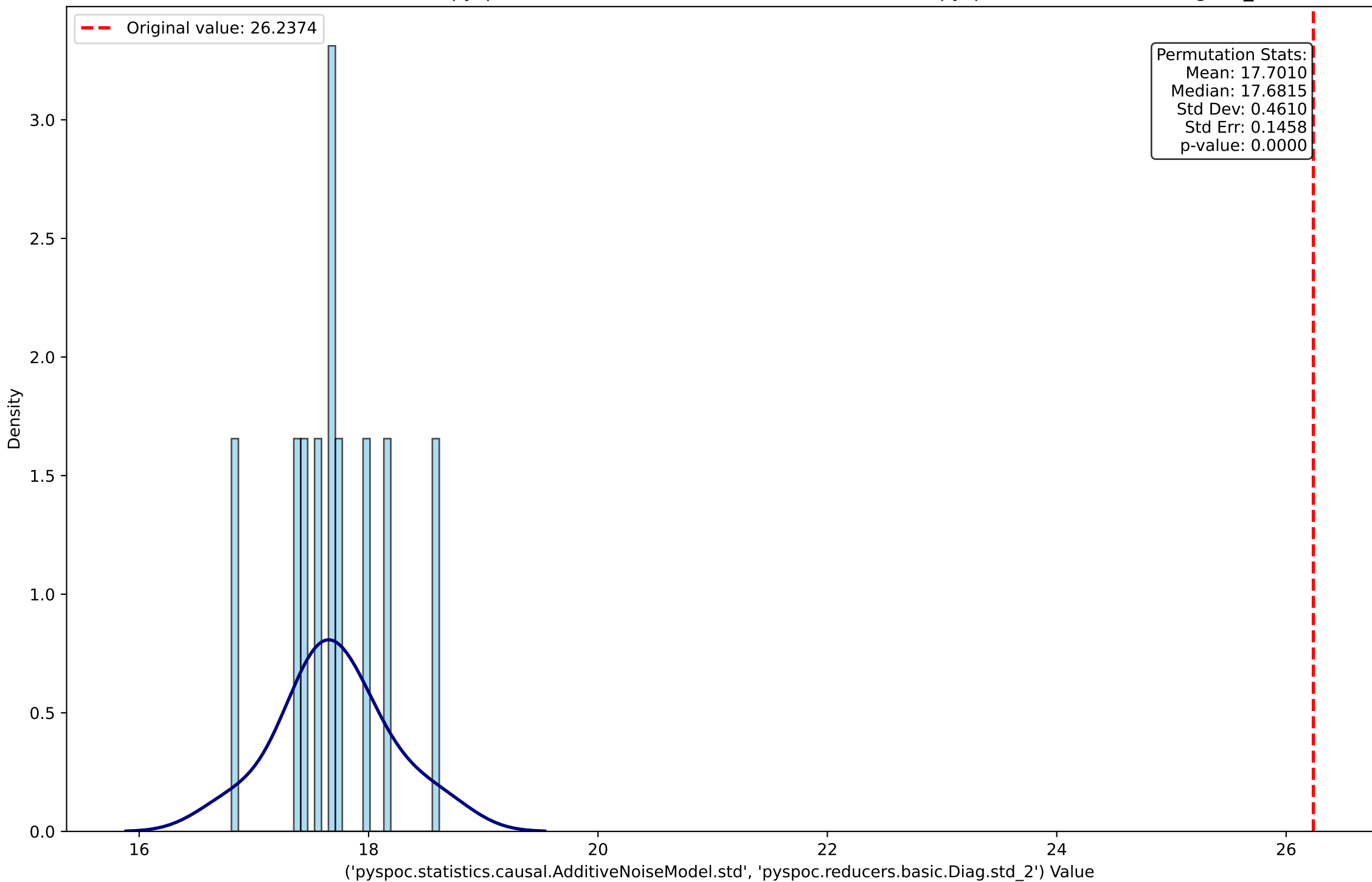
Permutation Distribution for ('pyspoc.statistics.causal.AdditiveNoiseModel.std', 'pyspoc.reducers.basic.Diag.std_2')
