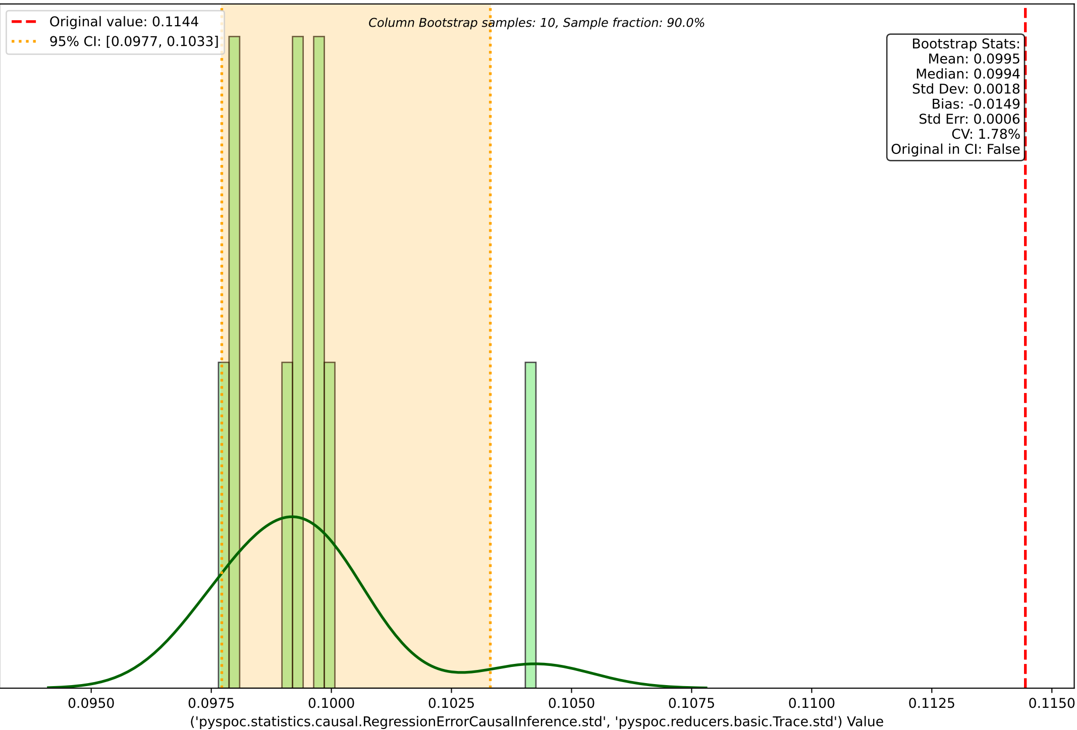
Column Bootstrap Distribution for ('pyspoc.statistics.causal.RegressionErrorCausalInference.std', 'pyspoc.reducers.basic.Trace.std')
