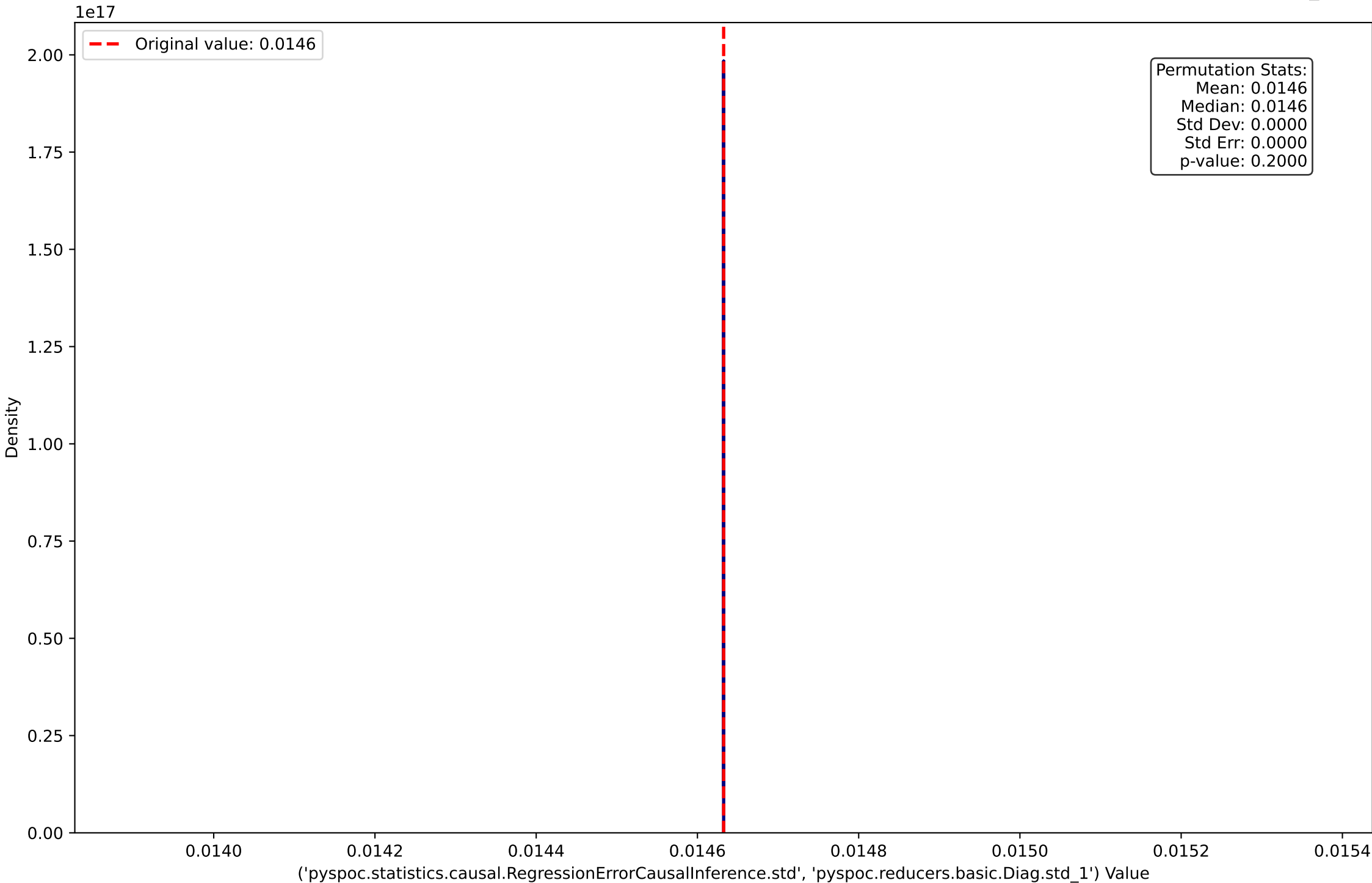
Permutation Distribution for ('pyspoc.statistics.causal.RegressionErrorCausalInference.std', 'pyspoc.reducers.basic.Diag.std_1')
