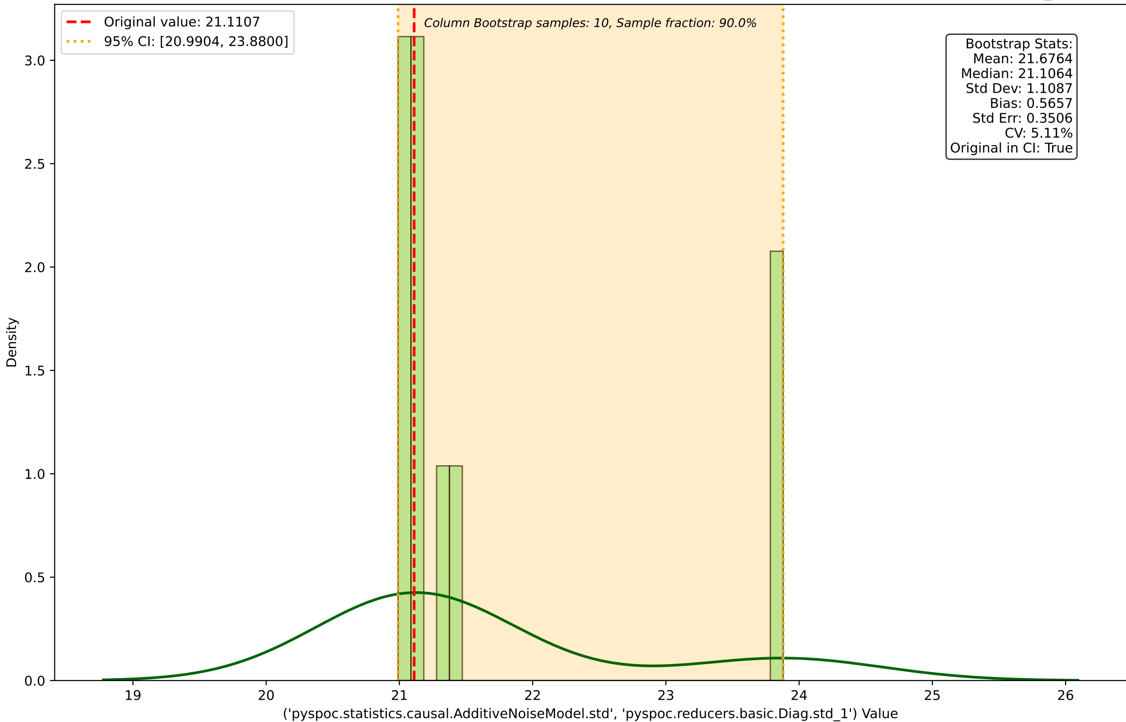
Column Bootstrap Distribution for ('pyspoc.statistics.causal.AdditiveNoiseModel.std', 'pyspoc.reducers.basic.Diag.std_1')
