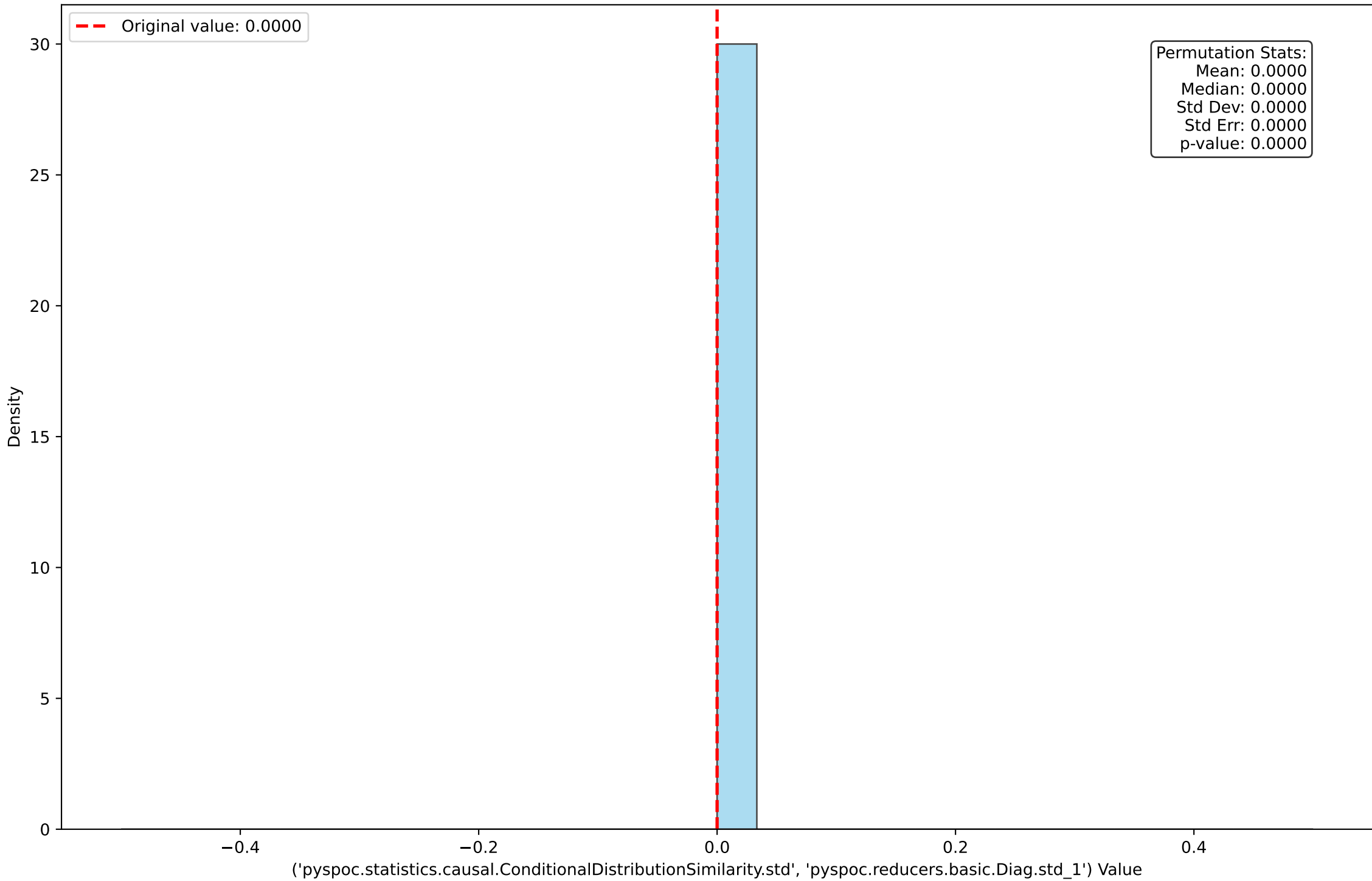
Permutation Distribution for ('pyspoc.statistics.causal.ConditionalDistributionSimilarity.std', 'pyspoc.reducers.basic.Diag.std_1')
