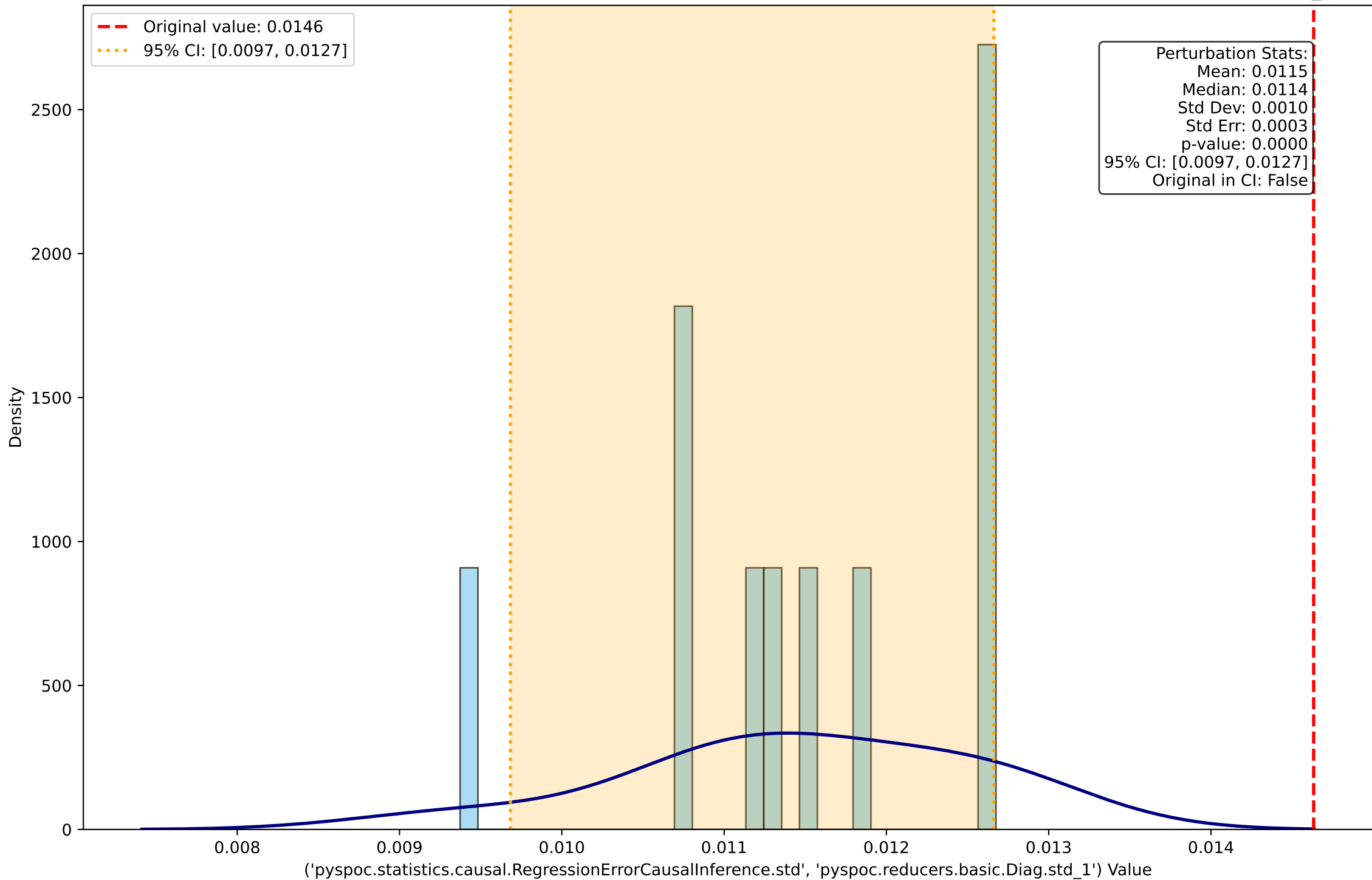
Perturbation Distribution for ('pyspoc.statistics.causal.RegressionErrorCausalInference.std', 'pyspoc.reducers.basic.Diag.std_1')
