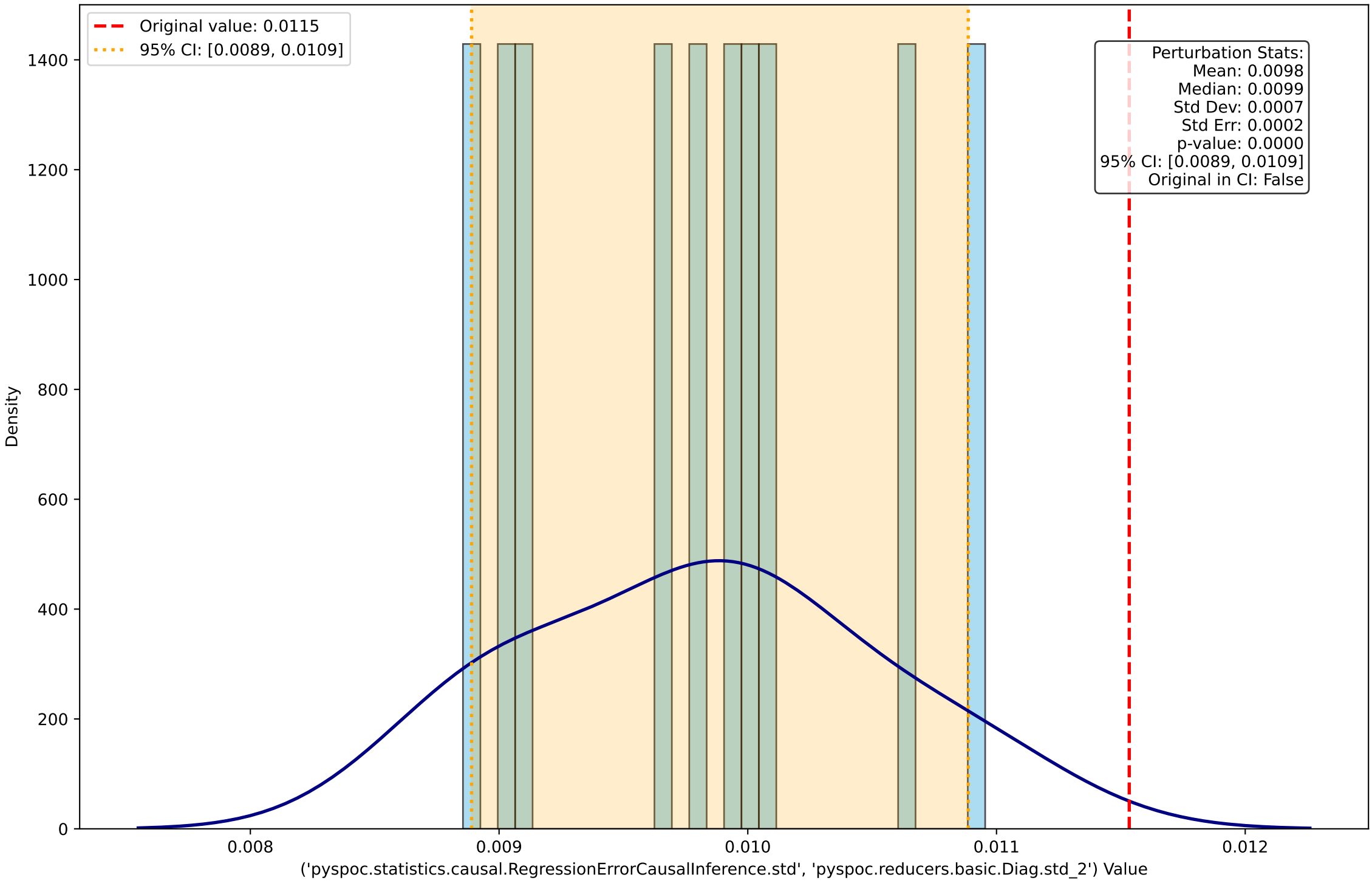
Perturbation Distribution for ('pyspoc.statistics.causal.RegressionErrorCausalInference.std', 'pyspoc.reducers.basic.Diag.std_2')
