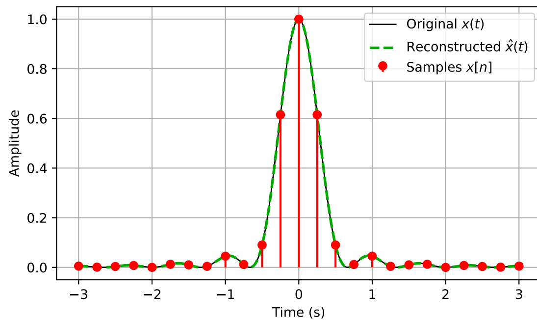
fs = 4.0 Hz - Reconstruction Status: Success
