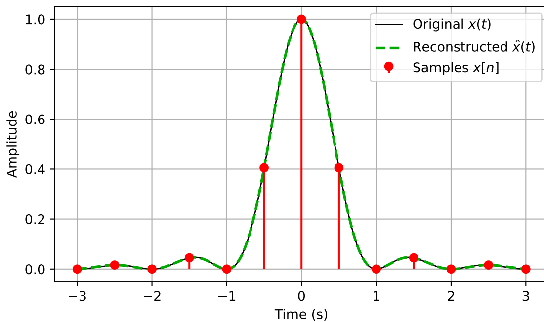
fs = 2.0 Hz - Reconstruction Status: Success
