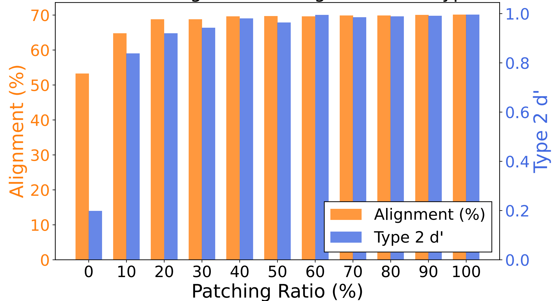
Effect of Patching Ratio on Alignment and Type 2 d'
