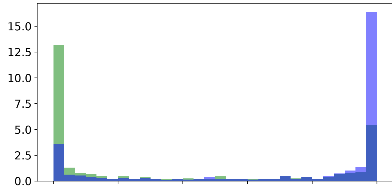
3B - Trained
