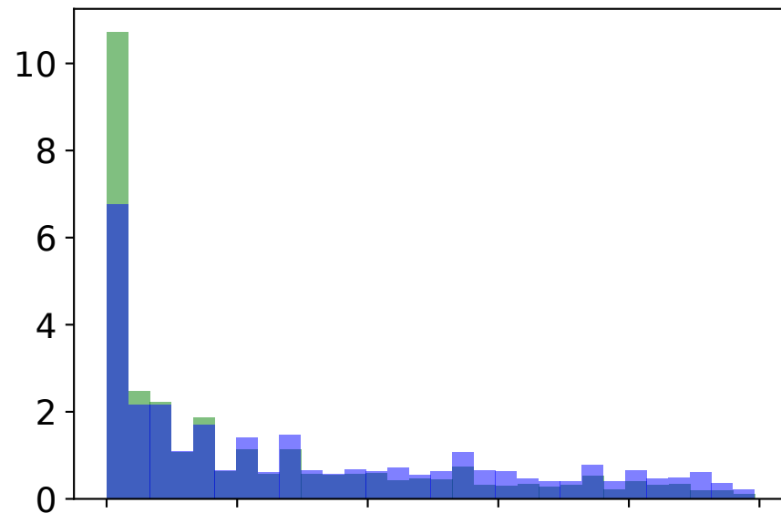
3B Base
