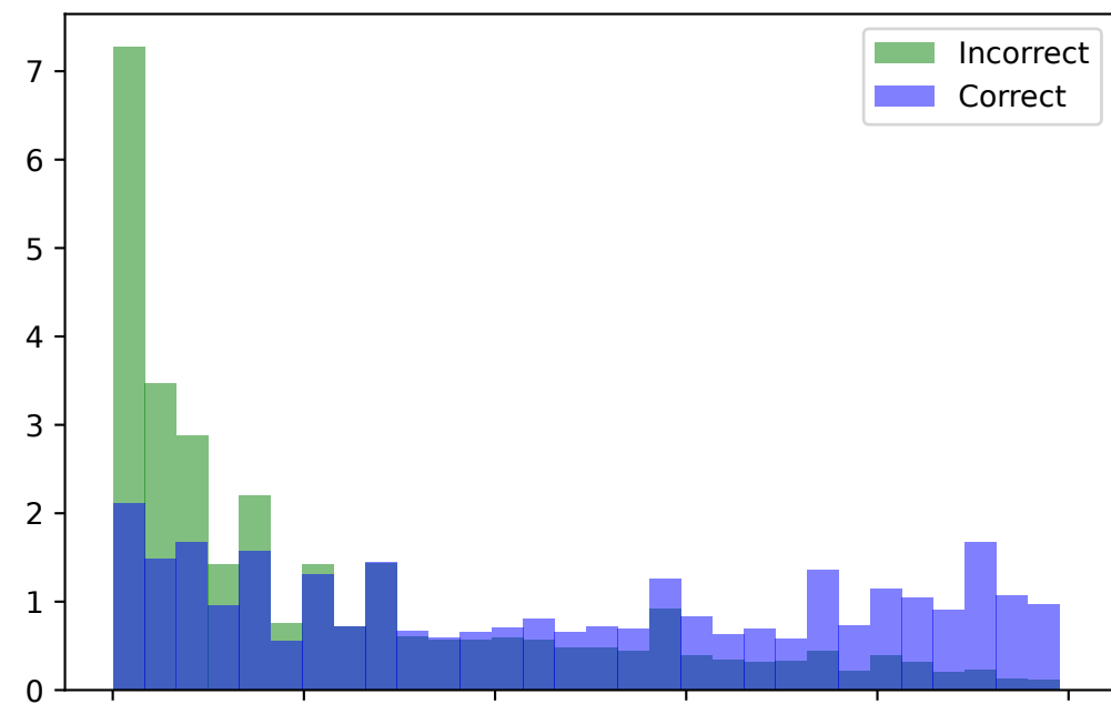
1.5B - Trained
