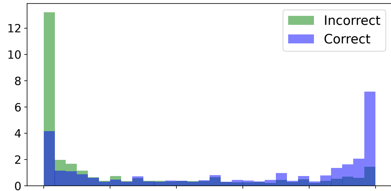
1.5B - Trained
