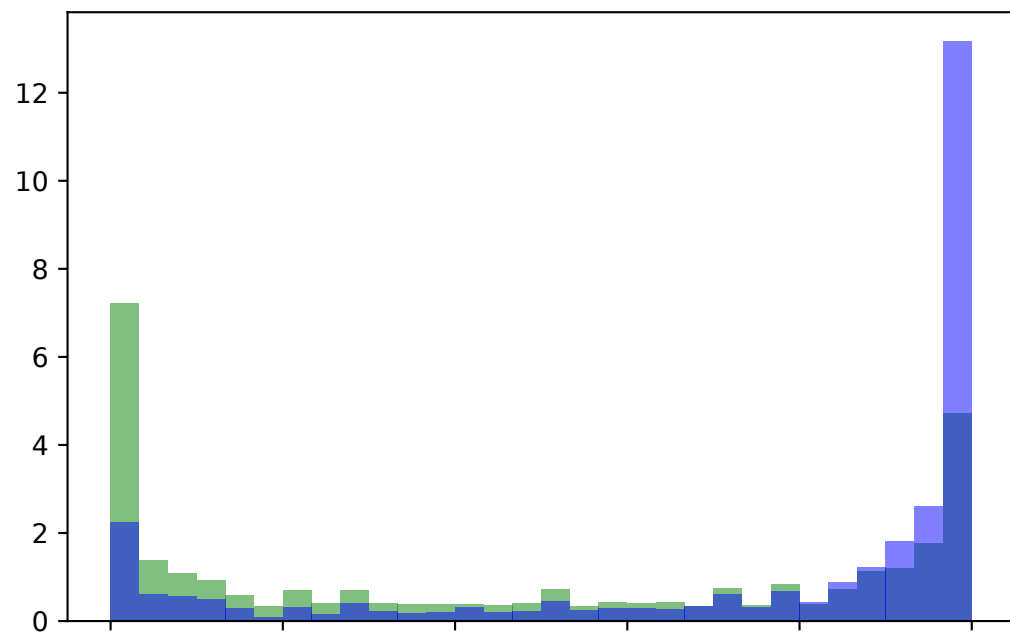
3B - Trained
