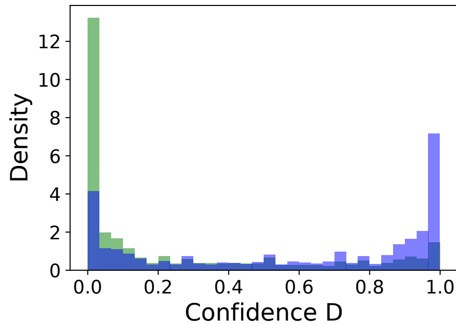
1.5B Fine-tuned
