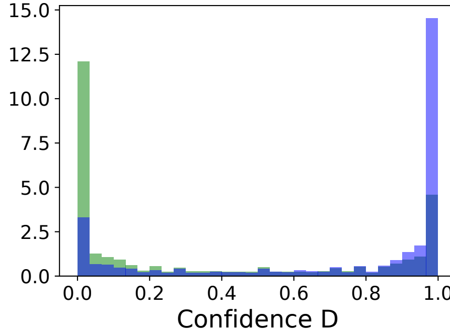
3B Fine-tuned
