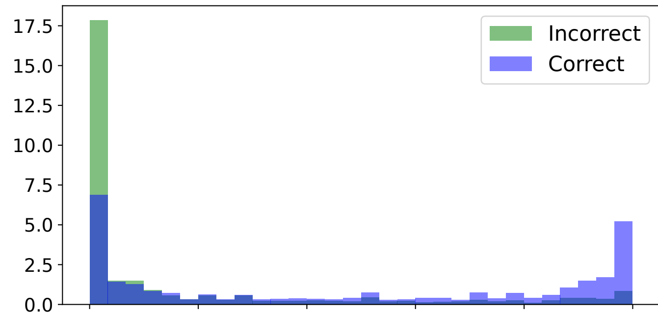
1.5B - Trained
