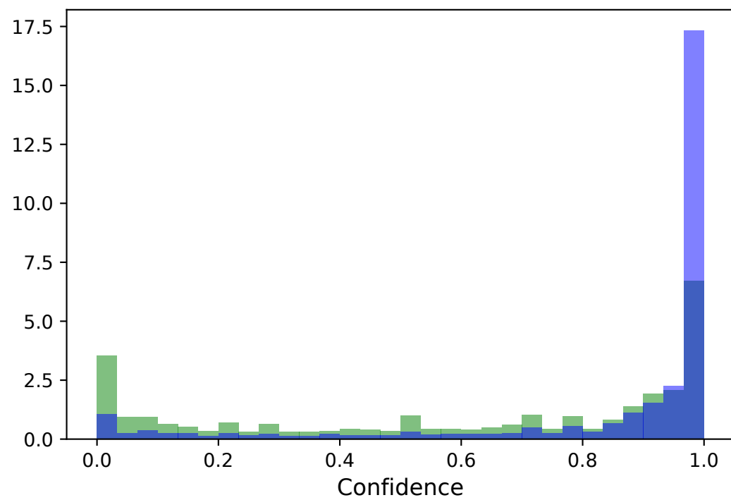
7B - Trained
