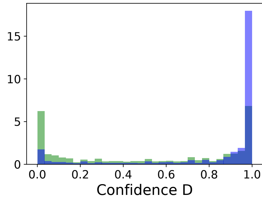
7B Fine-tuned
