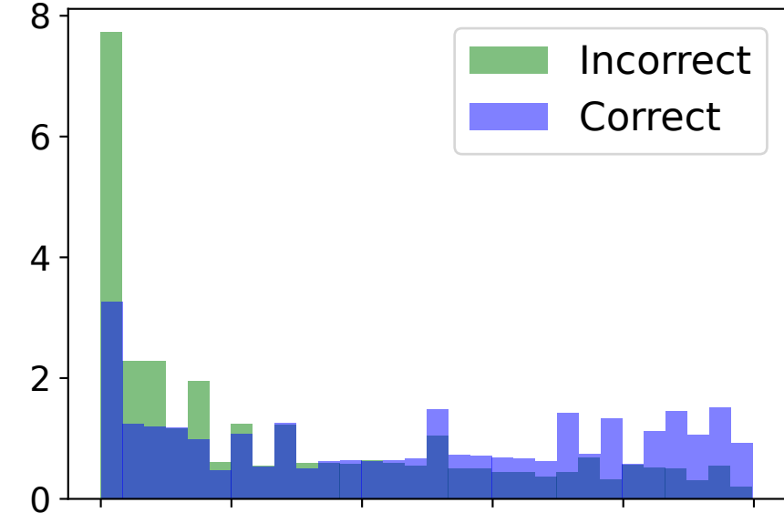
7B Base
