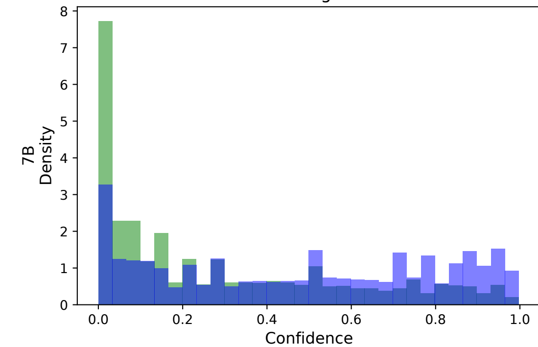
7B - Original
