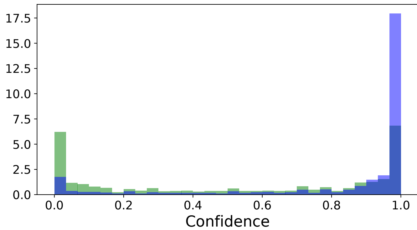
7B - Trained
