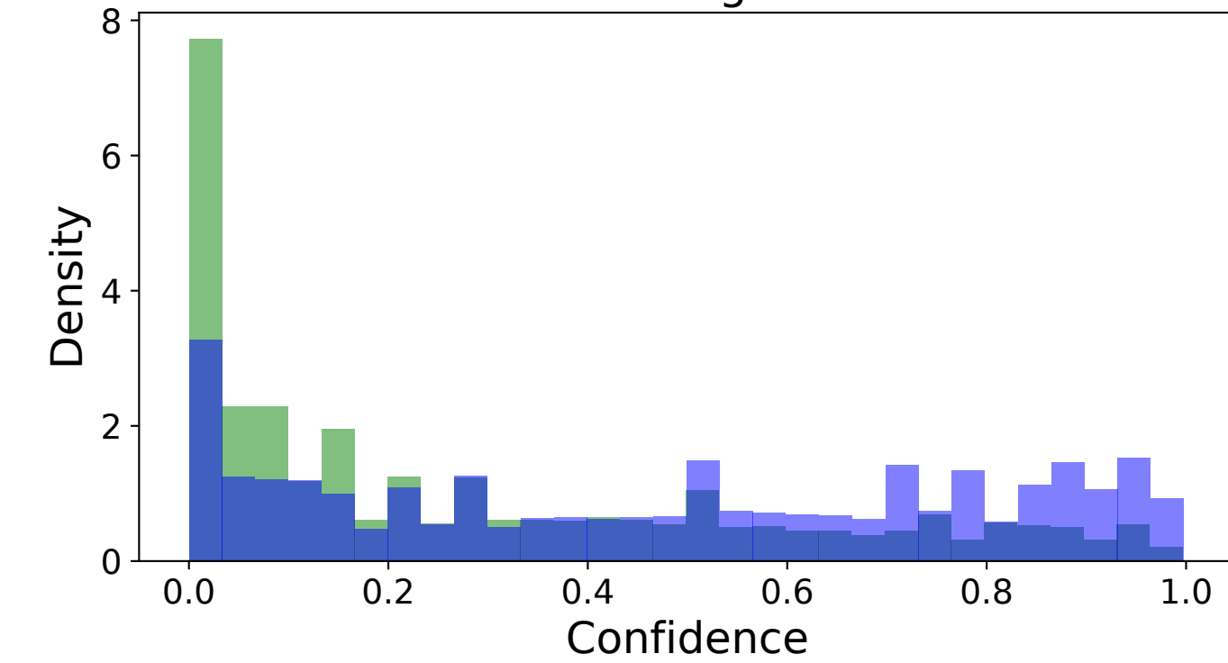
7B - Original
