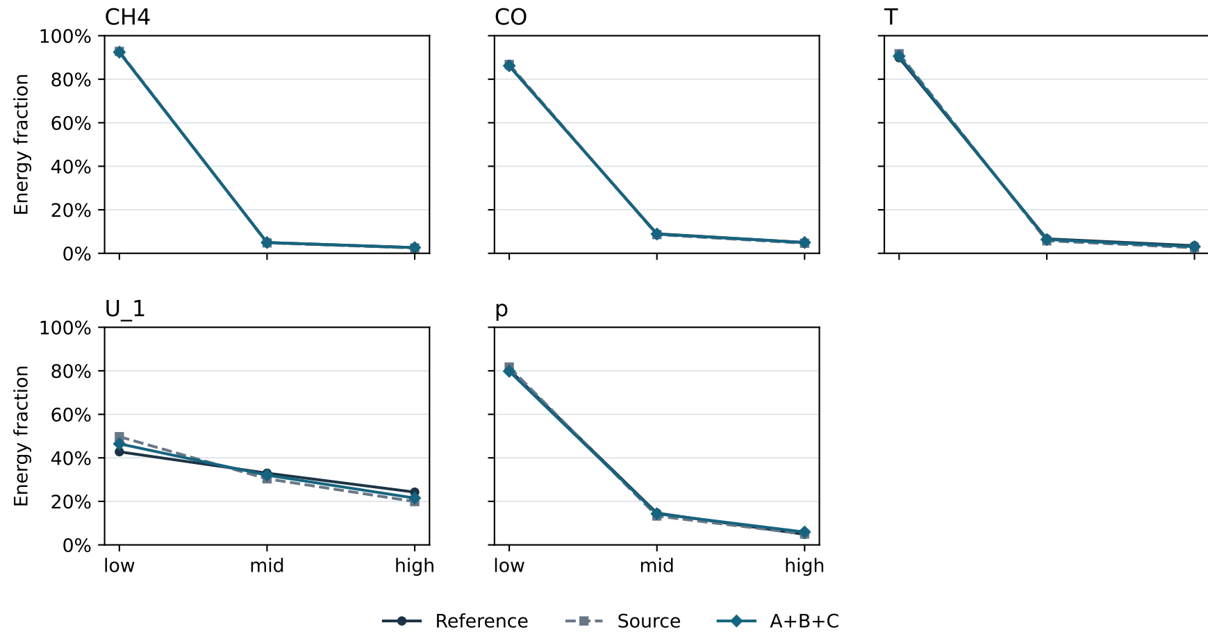
Graph-Fourier band energy · reference, source, A+B+C
