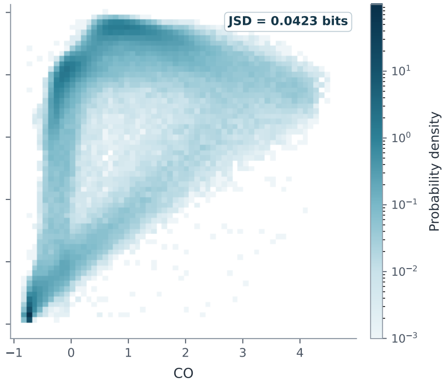
Reconstruction
