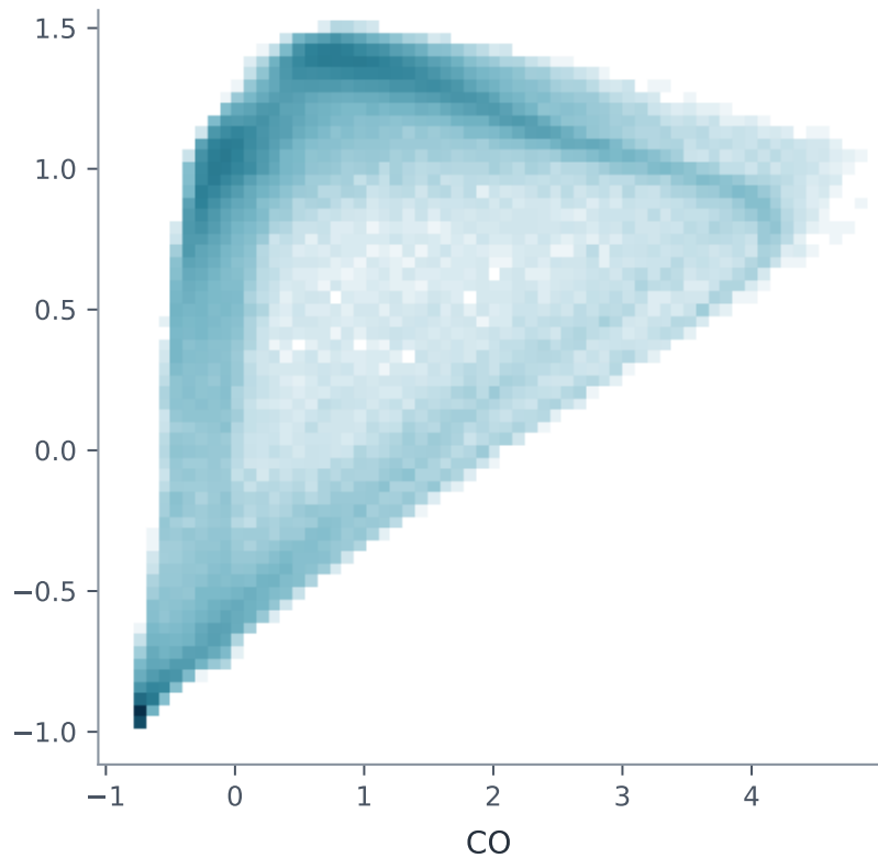
Ground truth
