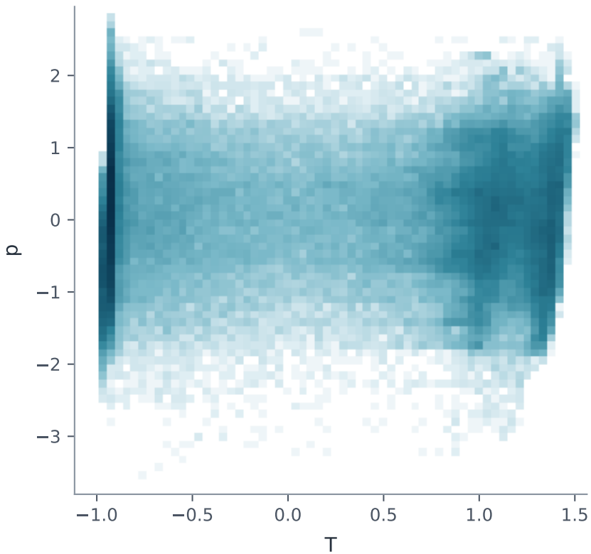
Ground truth
