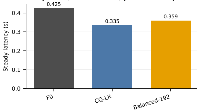
1M queries, Euler NFE=4, persistent Top-K
