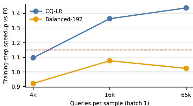
Balanced-192 never reaches 1.15x
