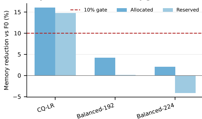
1M queries, Euler NFE=4, persistent Top-K
