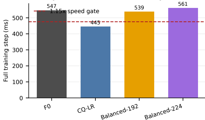
Balanced-192 never reaches 1.15x
