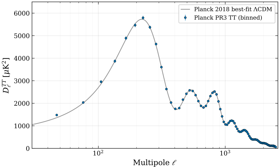
Planck PR3 TT power spectrum
