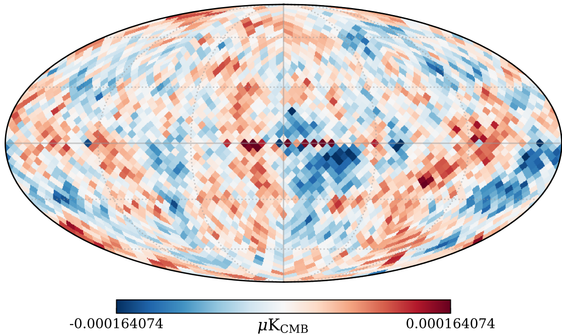
Planck Commander CMB \Delta T (NSIDE = 16)
