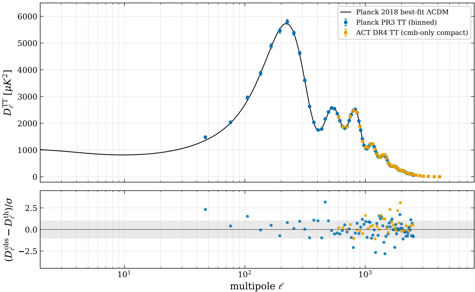
Multi-experiment CMB TT — Planck PR3 \cup ACT DR4 vs best-fit \Lambda CDM
