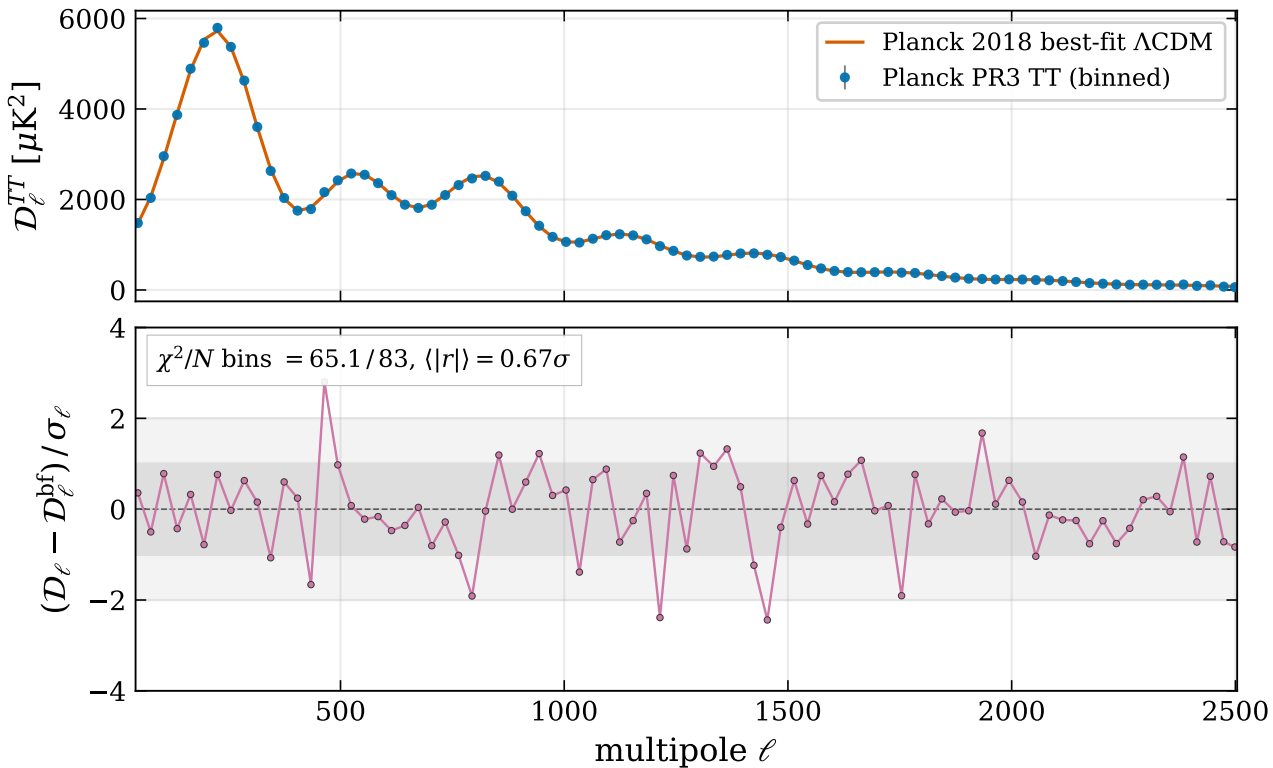
Planck PR3 TT bandpowers vs best-fit \Lambda CDM
