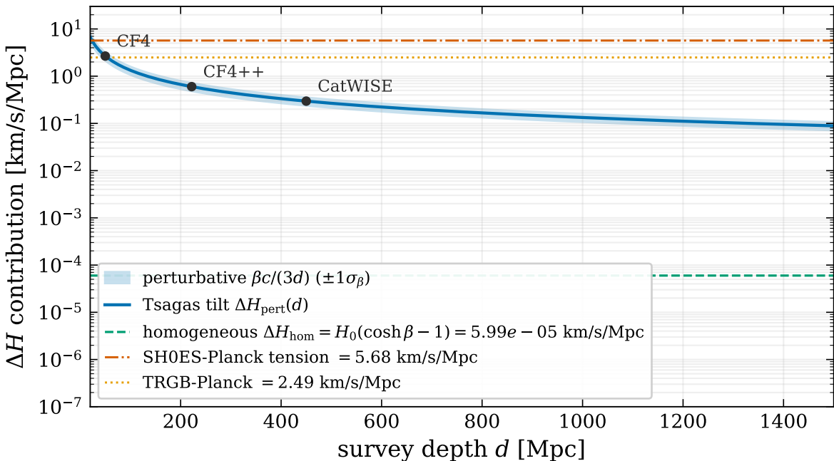
Tilt-induced \Delta H vs the H_0 tension: homogeneous (frame) and perturbative (peculiar) channels
